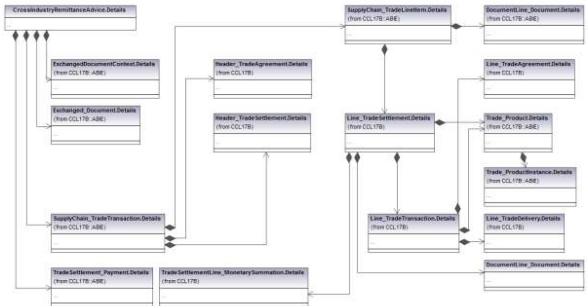
207 Figure 1 Cross Industry Remittance Advice conceptual data model
