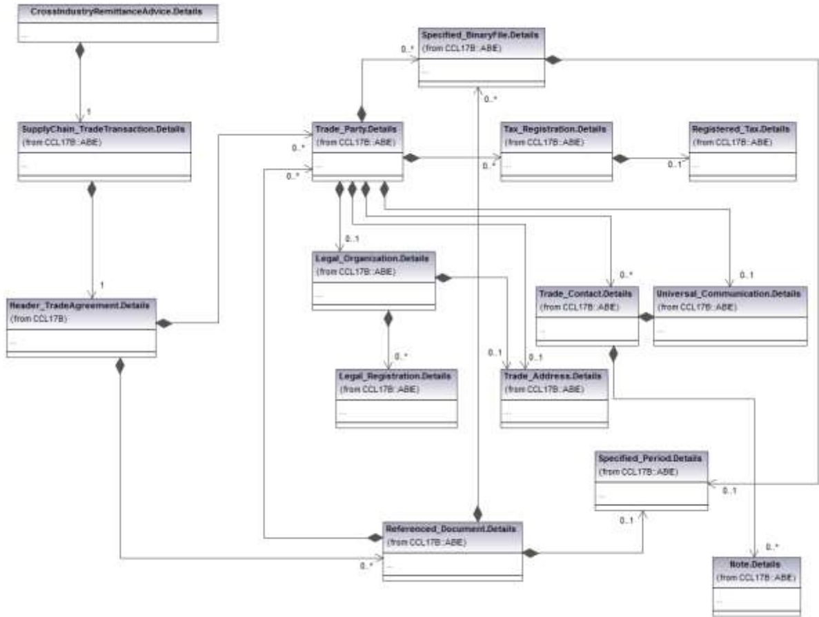
258 Figure 3 Header Trade Agreement
