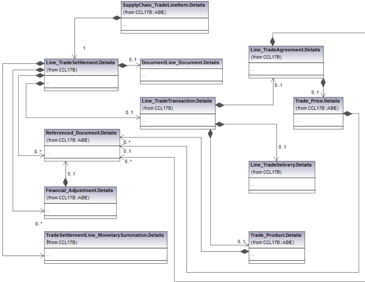
Figure 6 Line Trade Settlement
