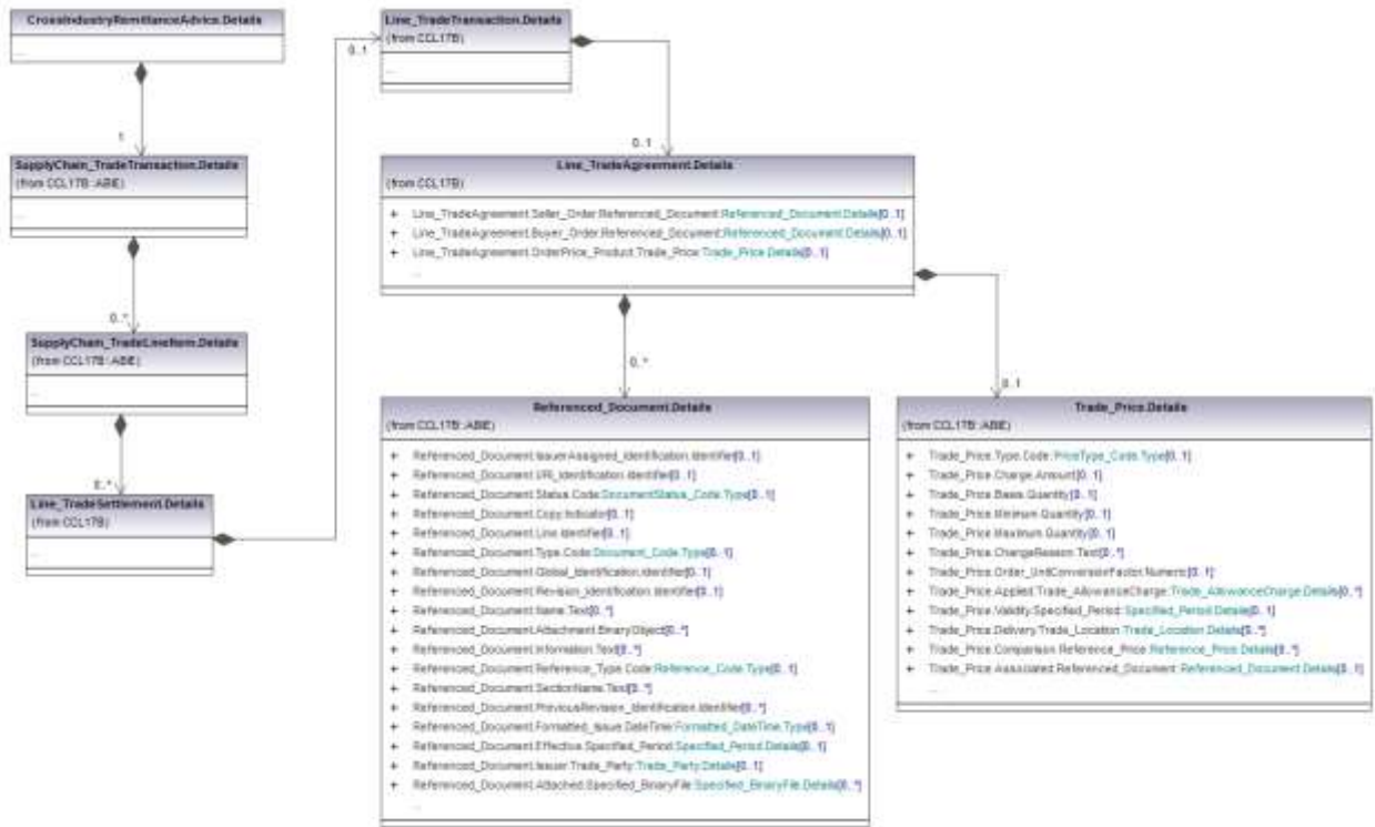
384 Figure 16 Line Trade Agreement 385
