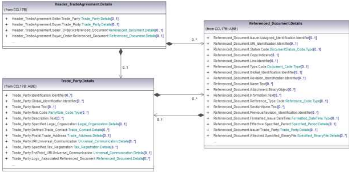
Figure 11 Header Trade Agreement
