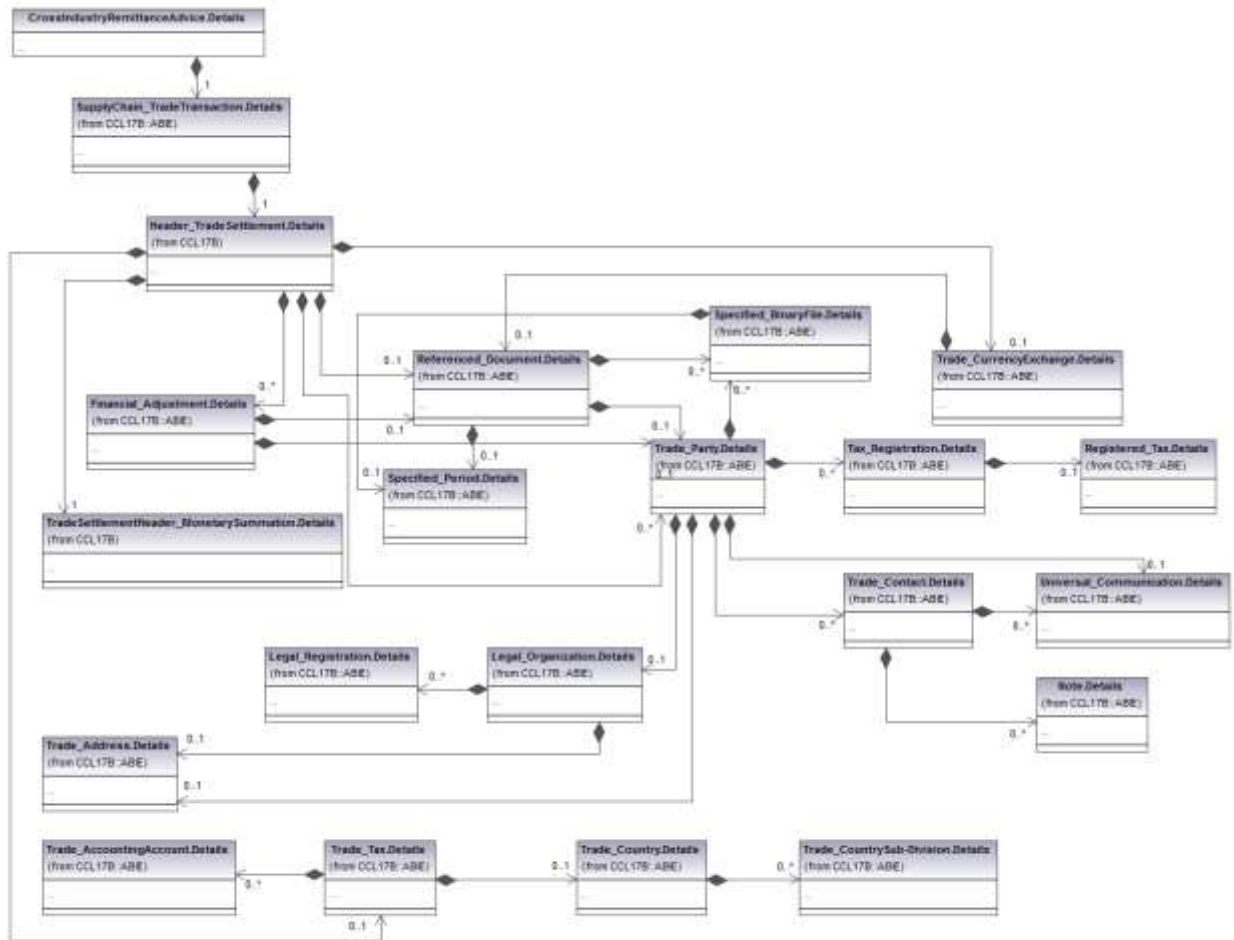
267 Figure 4 Header Trade Settlement
