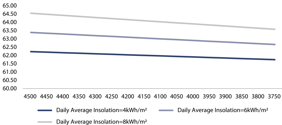
Figure 2 LCOE drop in response to solar system capital cost decline
