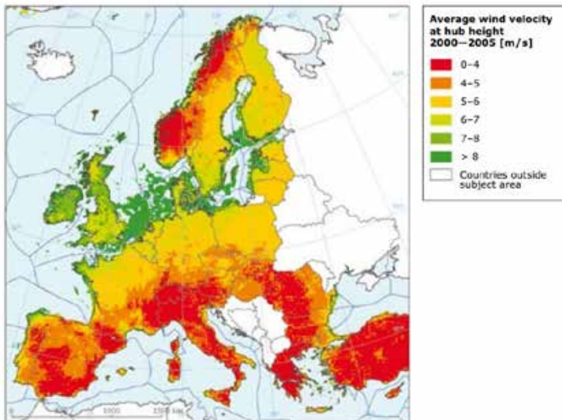
Figure 8 Average wind velocity at 80 metres height
