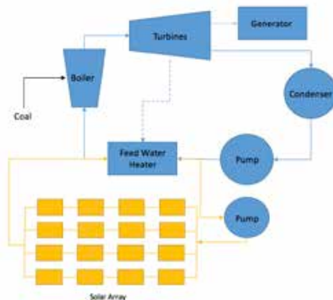
Figure 1 Model of SAPG preheat hybridization in a Rankine Cycle
