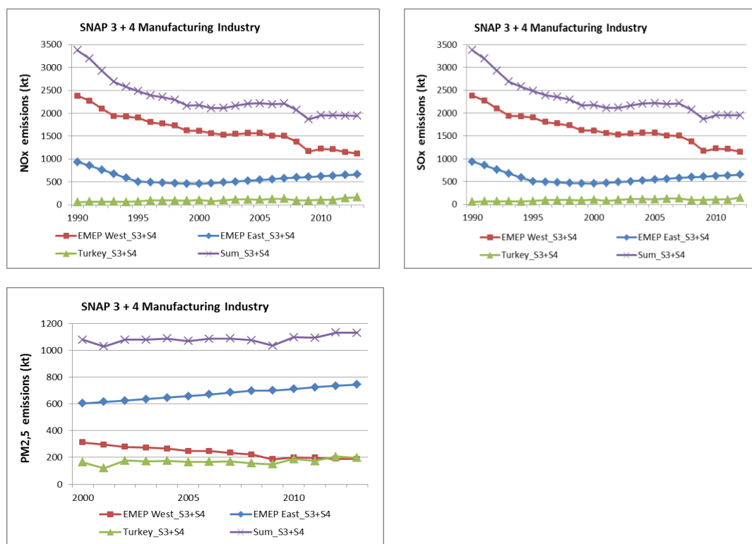
Figure C.6: NO x , SO x and PM 2.5 emission trends in manufacturing industries (S3+S4). Source: EMEP/CEIP data, 1990-2013
