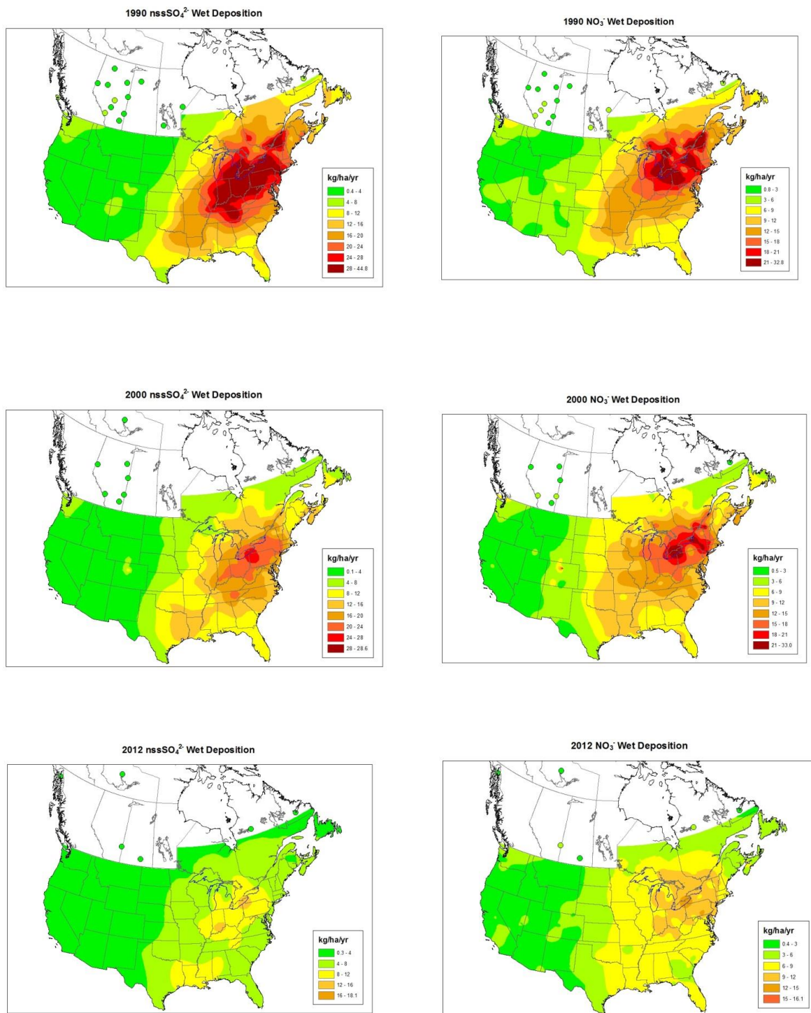
Figure 3.9: 1990-2012 Annual wet sulphate and wet nitrate deposition in North America (Source: National Atmospheric Chemistry Database (NAtChem) Database ( www.ec.gc.ca/natchem ) and National Atmospheric Deposition Program ( nadp.isws.illinois.edu ), 2016)
