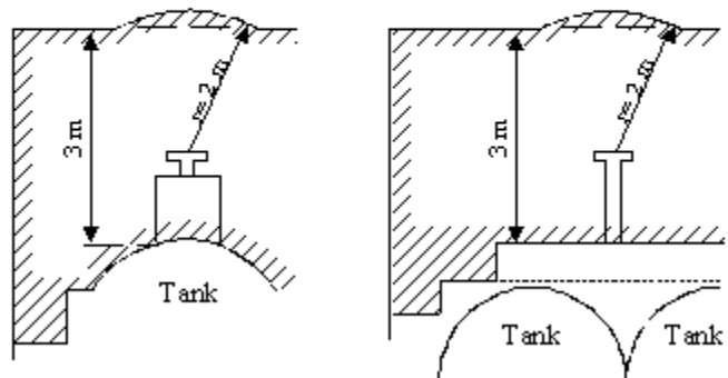
Tank vessels with independant cargo tanks
