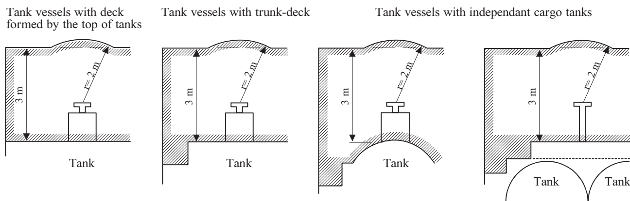
Above deck cargo area for various tank vessel
