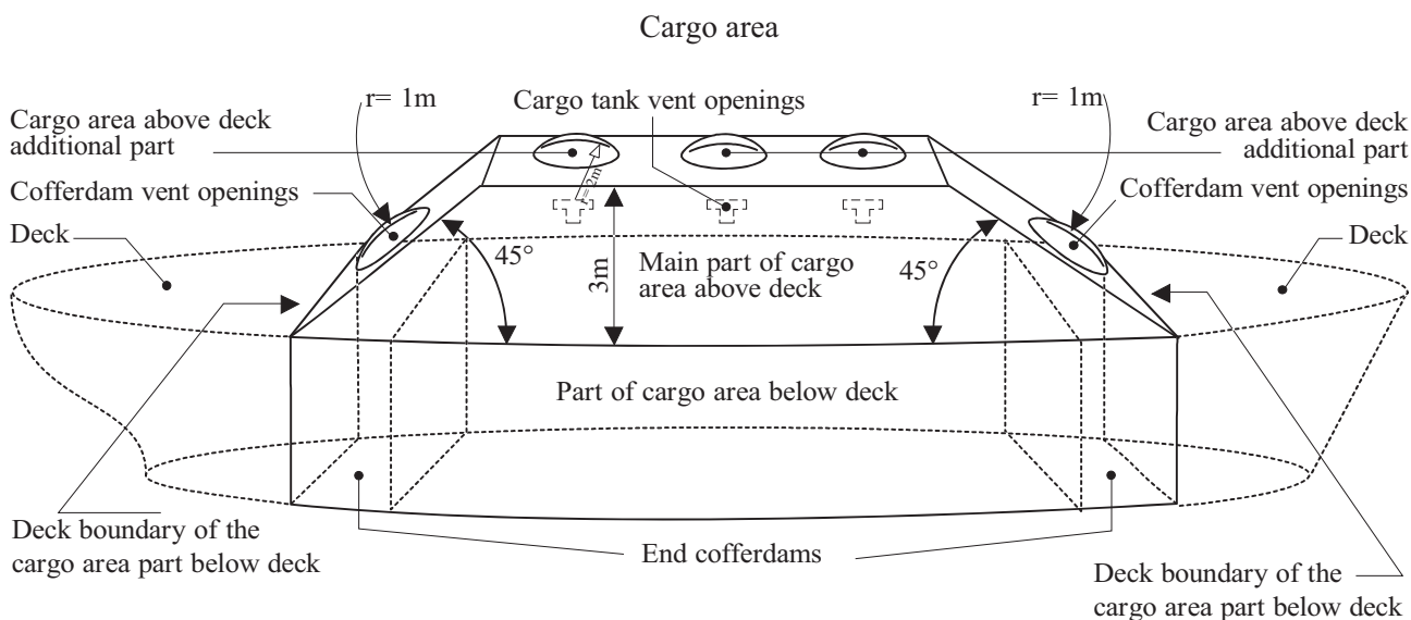
Above deck cargo area for various tank vessel
