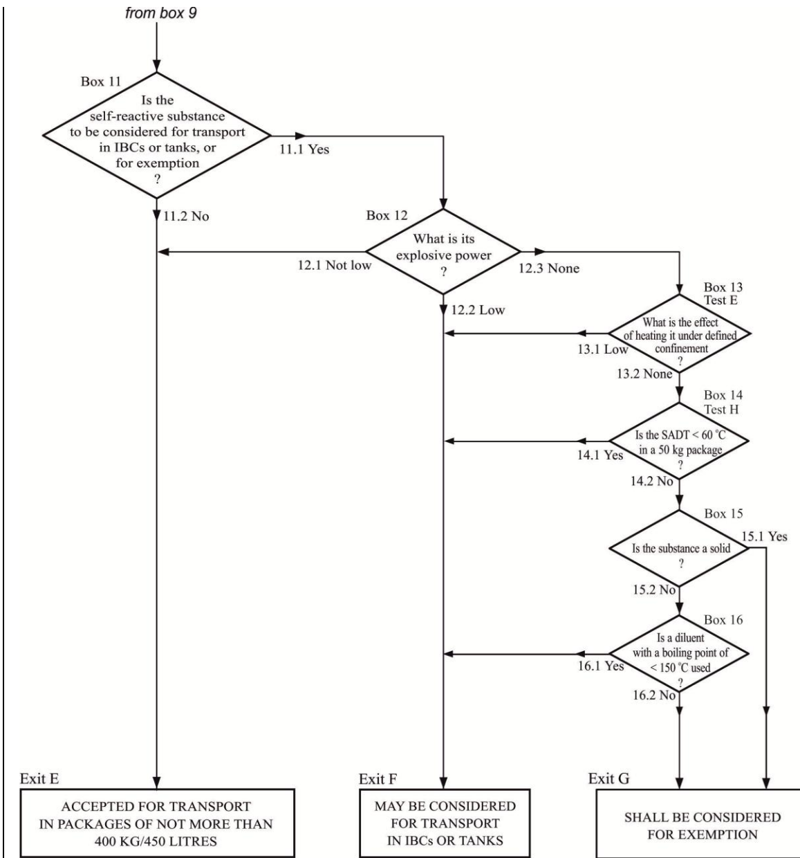
Figure 2.4.1: FLOW CHART SCHEME FOR SELF-REACTIVE SUBSTANCES (cont'd)
