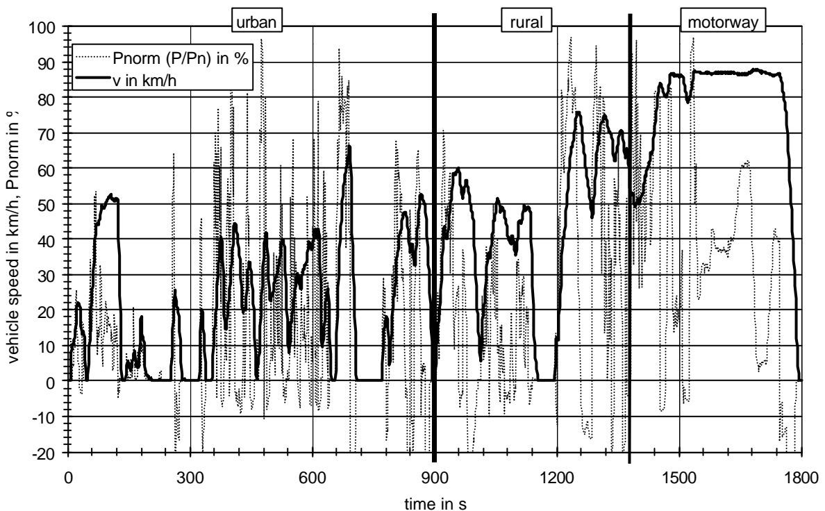
Figure 1 : The world-wide transient vehicle cycle (WTVC)
