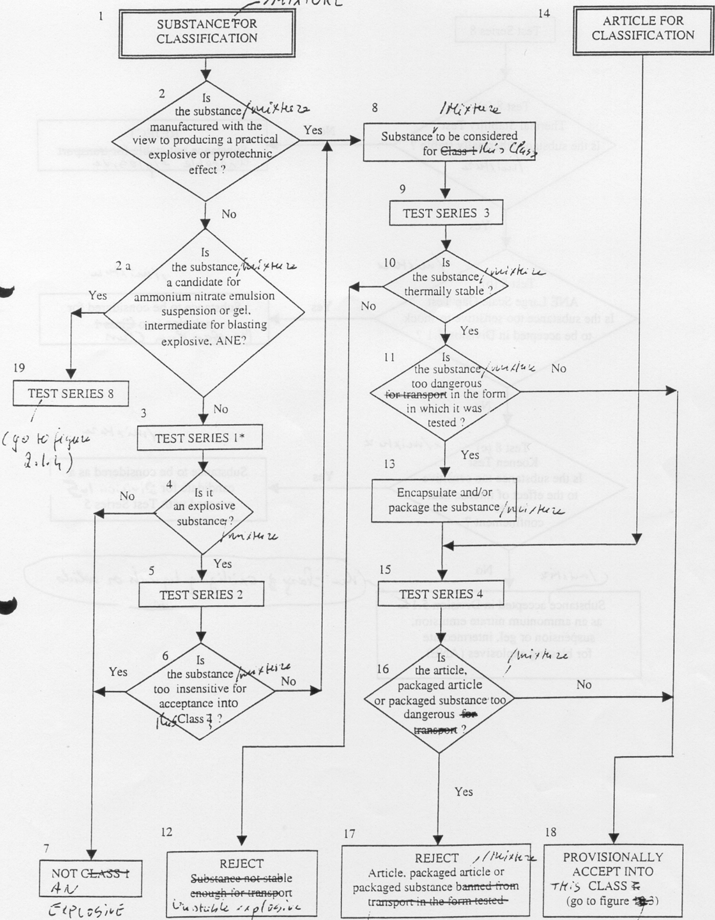
Figure 10.2: PROCEDURE FOR PROVISIONAL ACCEPTANCE OF A SUBSTANCE OR MIXTURE OR ARTICLE IN CLASS 1 THE CLASS OF EXPLOSIVES
