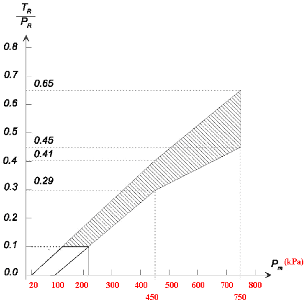
DIAGRAM 4A SEMI-TRAILERS (see paragraph 4. of this annex)
