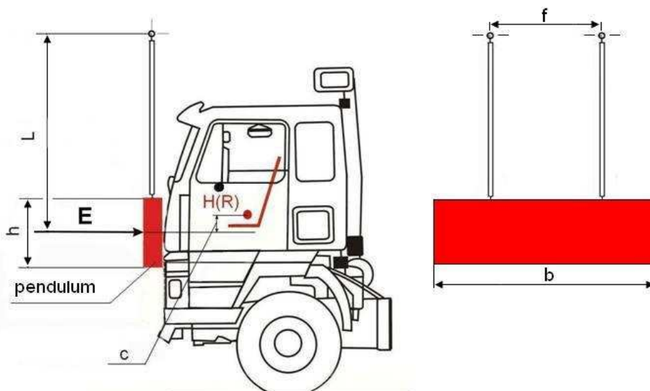
Fig. 1 – Front impact test (test A).
