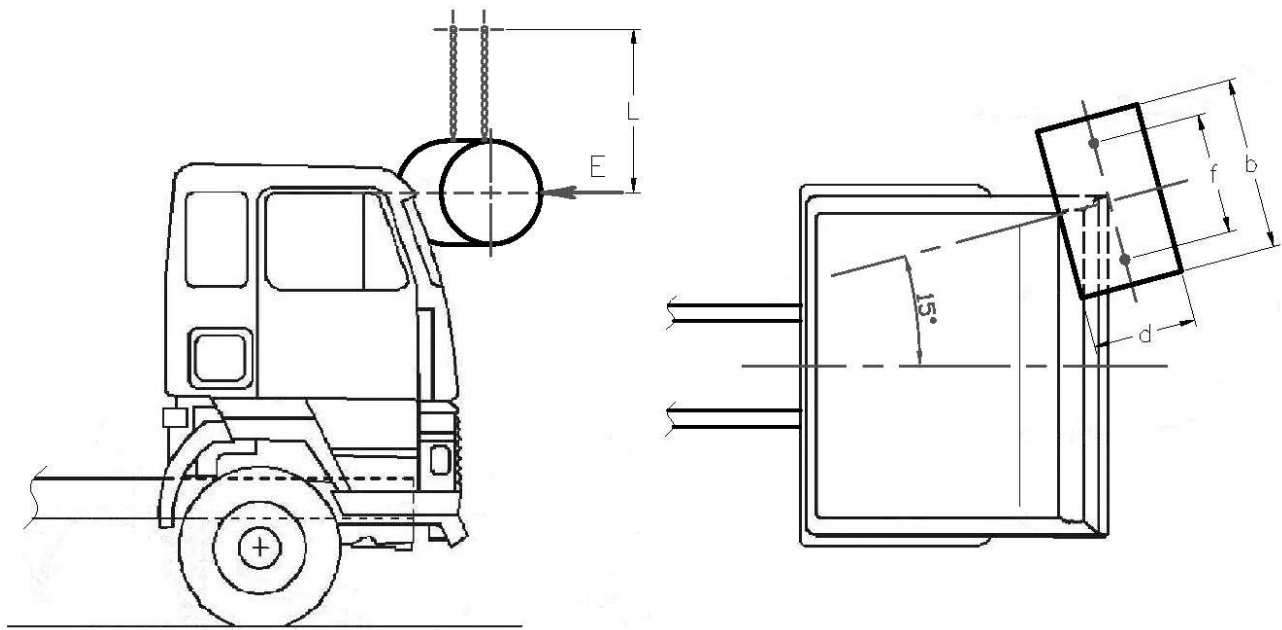
Fig. 2. – Front pillar impact test (Test B).
