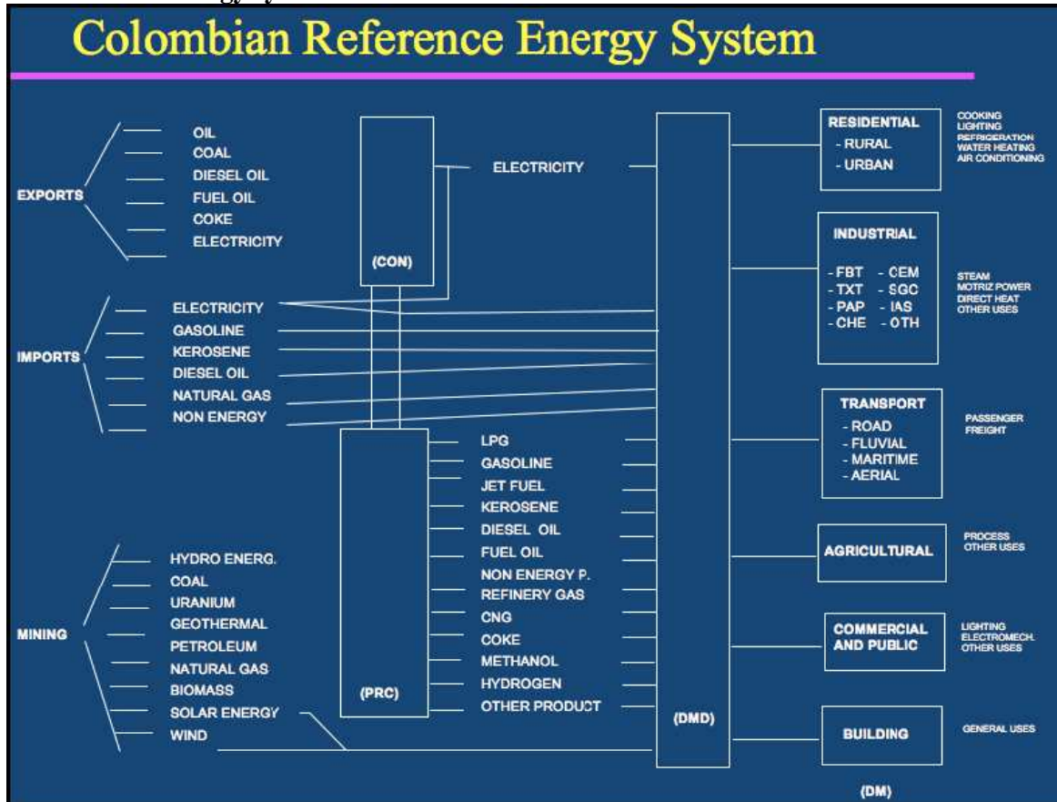
Figure 5: The reference energy system considered in MARKAL-Colombia
