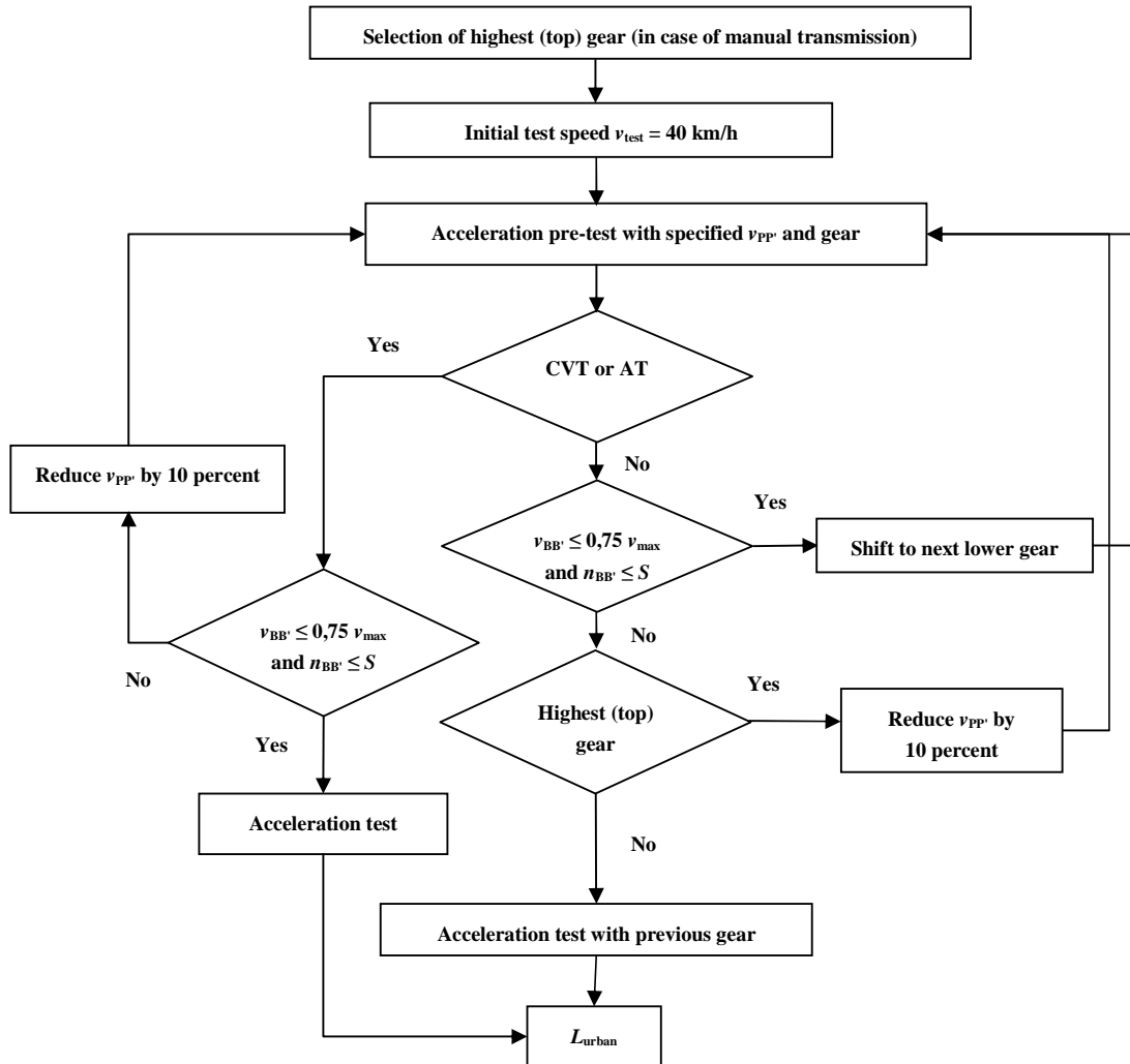
Flowchart of the test procedure for the test of the vehicle in motion for vehicles of category L_3 with PMR \leq 25
