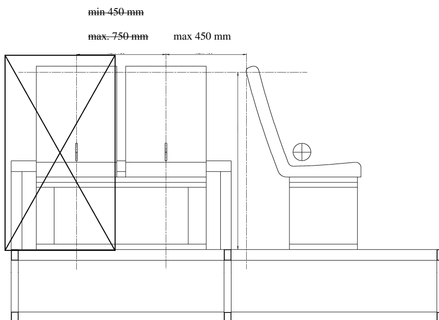
Figure 1: Positioning requirements for side-facing seats
