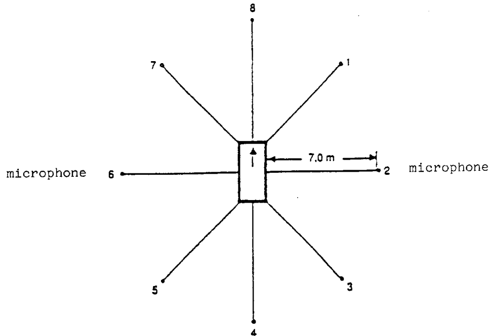
Figure 1: Microphone positions for measurement of compressed air sound noise
