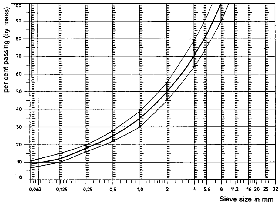
Figure 2: Grading curve of the aggregate in the stone asphaltic mix with tolerances.
