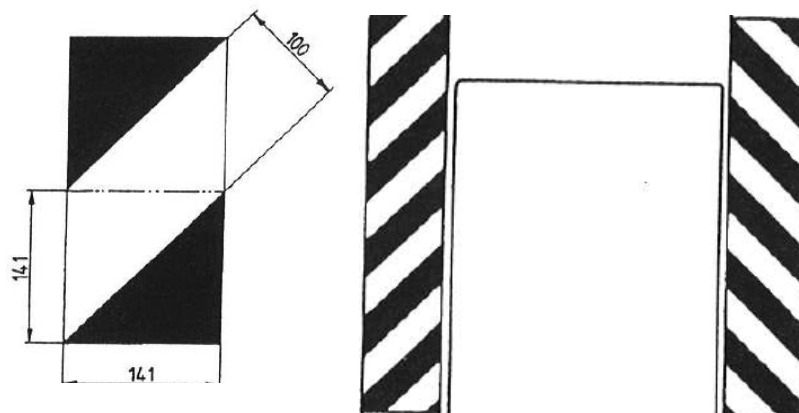
Figure 3a Retro-reflective material marking of class F
