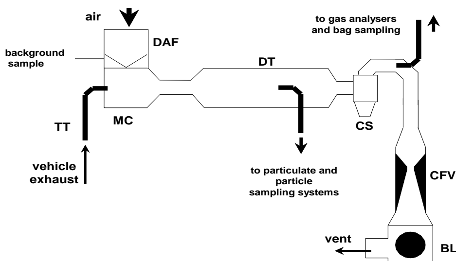
Figure A4a.App2/7 Critical-Flow Venturi Dilution System
