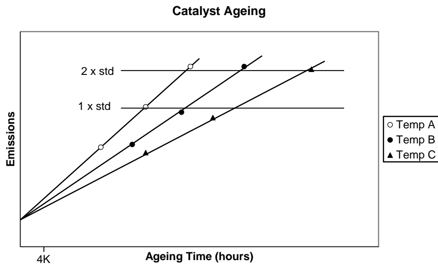
Figure A9.App1/3: Example of catalyst ageing
