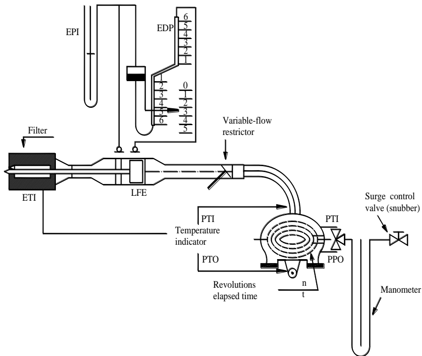
Figure A4a.App2/8 PDP Calibration Configuration
