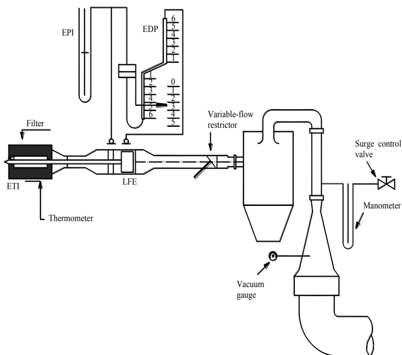
Figure A4a.App2/9 CFV Calibration Configuration
