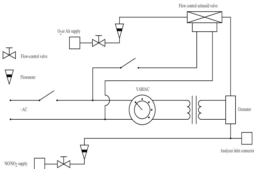
Figure A4a.App3/11 NO x Converter Efficiency Test Configuration
