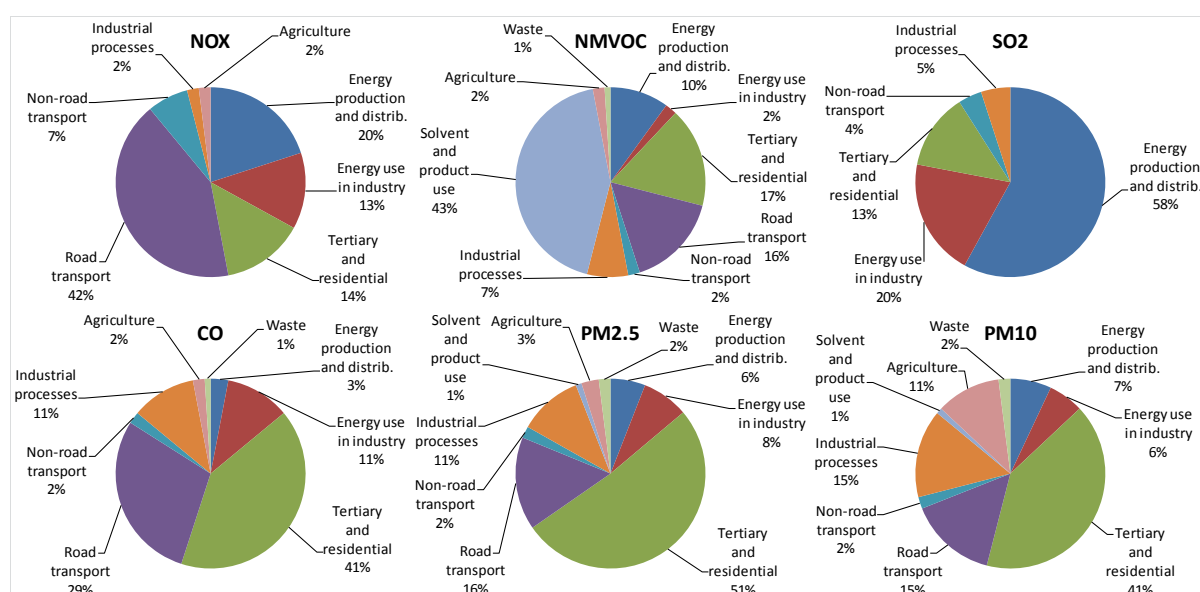
Figure 3. Share of emissions of the main pollutants by economic sector in the EU-27
