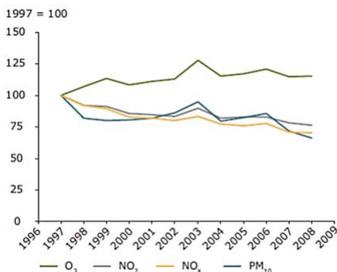
Figure 6. Indexed trends in air quality
