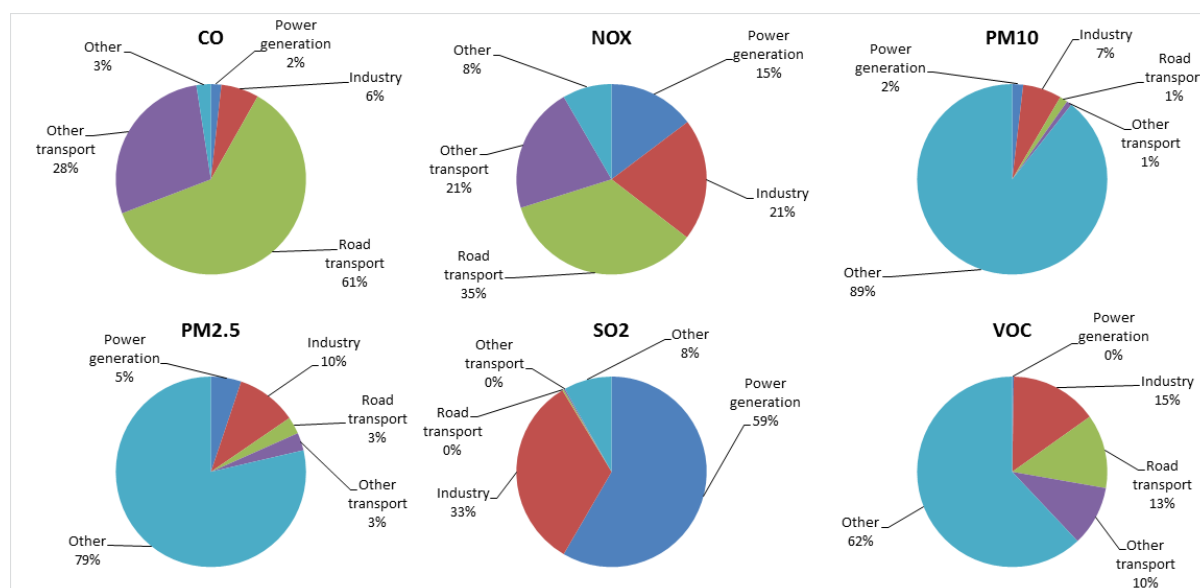
Figure 4. Share of emissions of the main pollutants by economic sector in the United States
