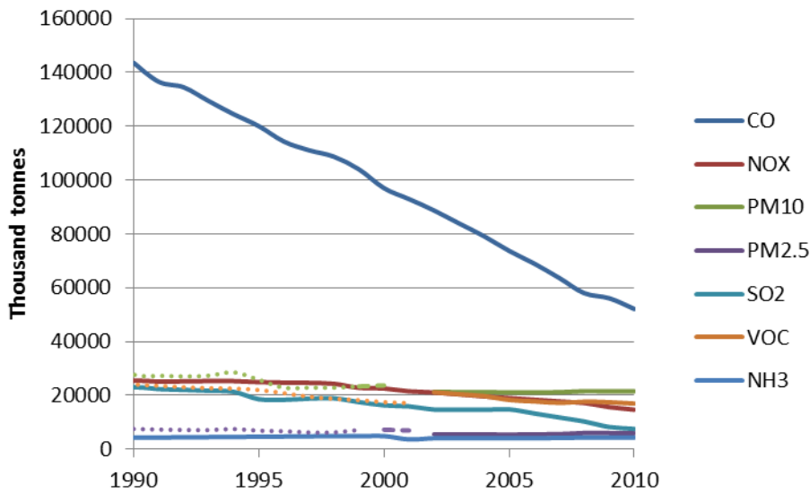
Figure 2. Air pollutant emissions trends in the United States
