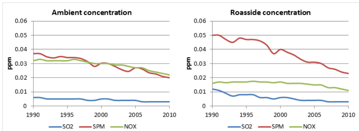
Figure 5. Atmospheric concentration SO 2 , suspended particulate matter and NO x in Japan
