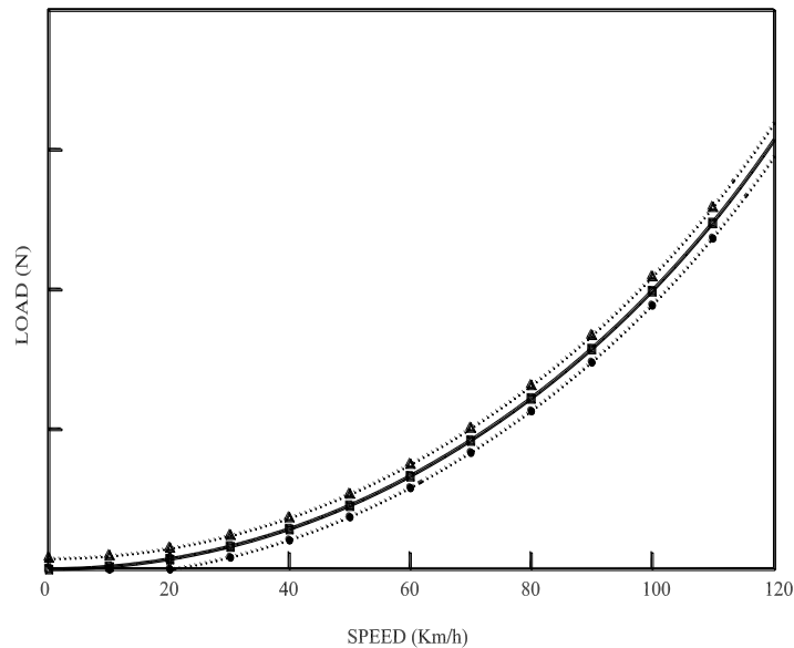
Figure A4a.App1/4 Diagram illustrating the power absorbed by the chassis dynamometer
