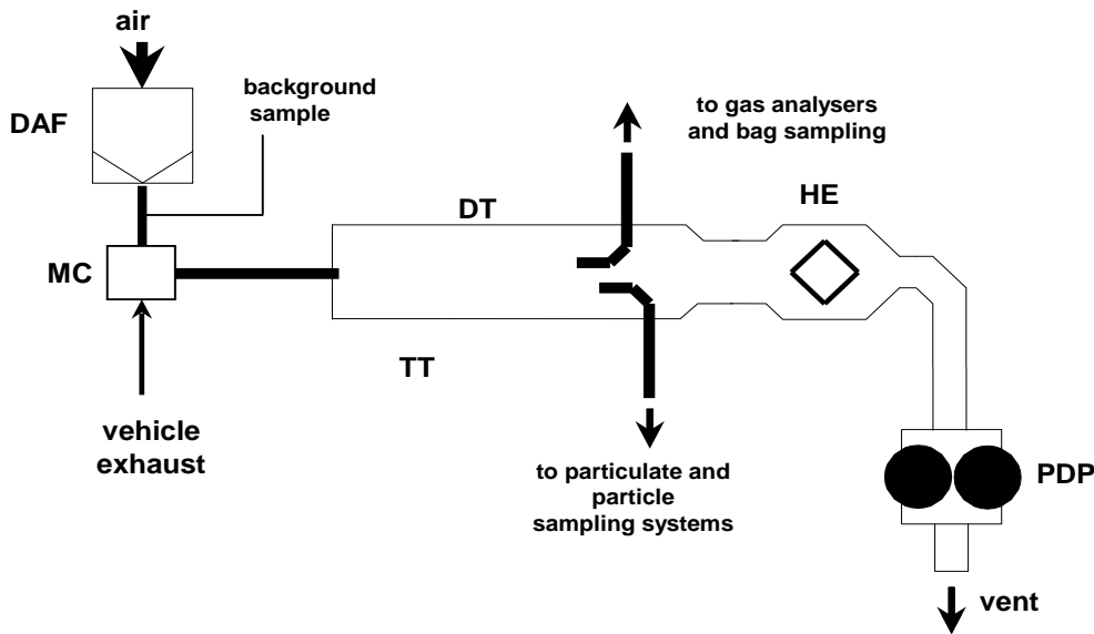
Figure A4a.App2/6 Positive Displacement Pump Dilution System
