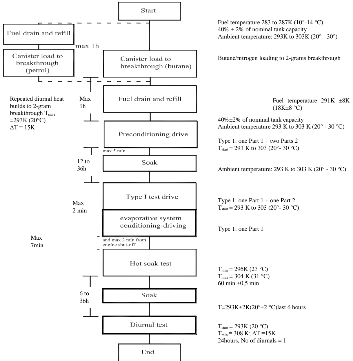
Figure A7/1 Determination of evaporative emissions 3000 km run-in period (no excessive purge/load) Ageing of canister(s) verified Steam-clean of vehicle (if necessary)
