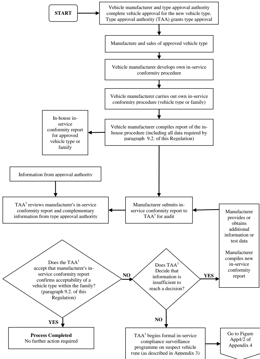
Figure App4/1 In-service conformity checking - audit procedure
