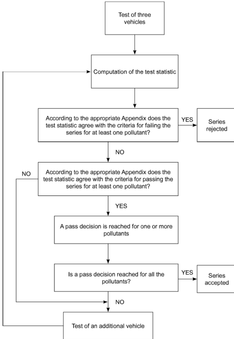
Figure 2 Checking the conformity of the vehicle
