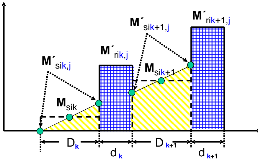
Figure A13/3 Parameters measured during emissions test during and between cycles where regeneration occurs (schematic example)
