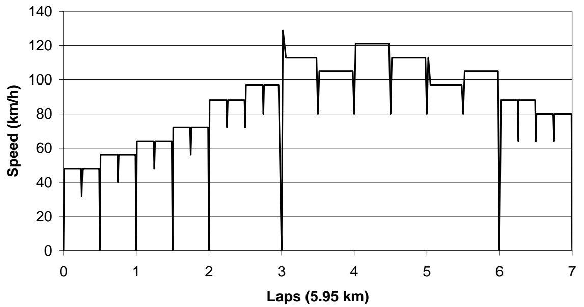
Standard Road Cycle
