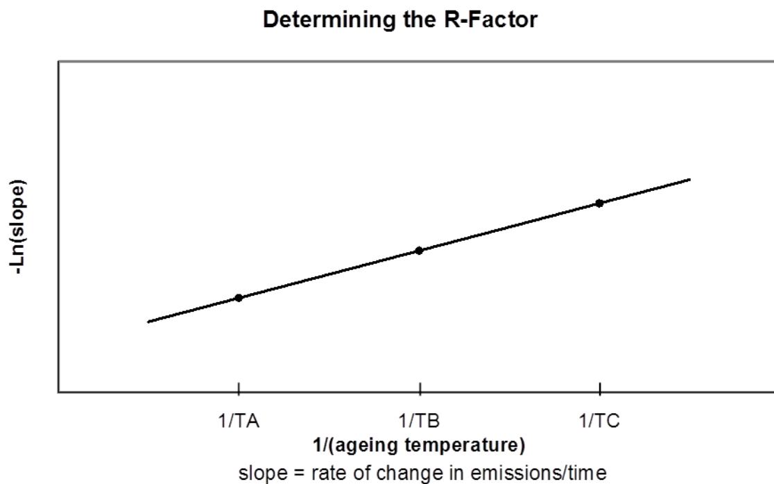
Figure A9.App1/4 Determining the R-Factor
