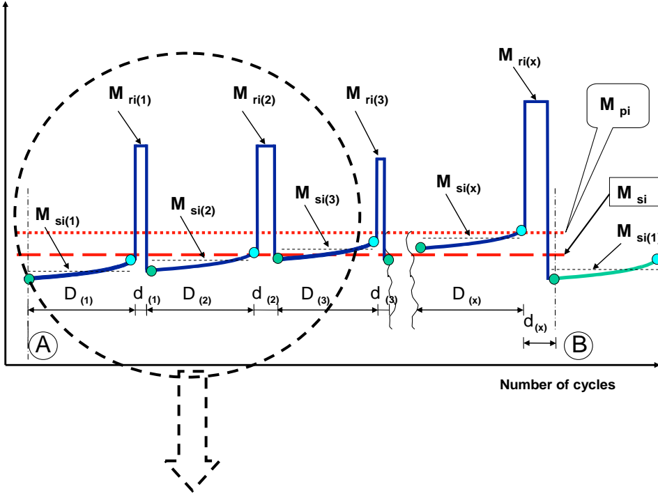
Figure A13/2 Parameters measured during emissions test during and between cycles where regeneration occurs (schematic example)
