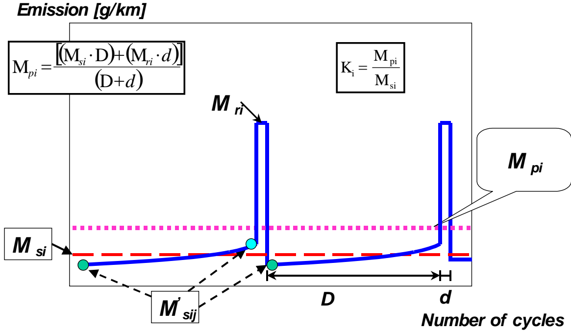
Figure A13/1 Parameters measured during emissions test during and between cycles where regeneration occurs (schematic example, the emissions during "D" may increase or decrease)
