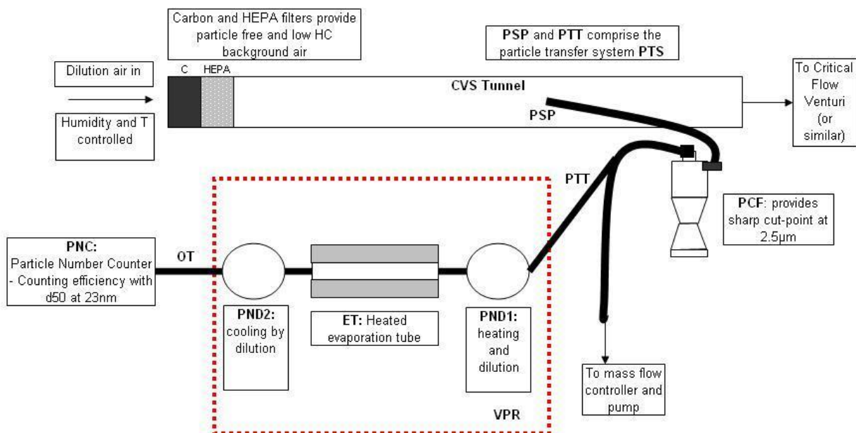
Figure A4a.App5/14 Schematic of Recommended Particle Sampling System
