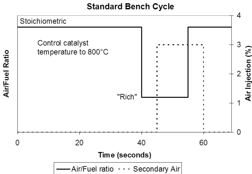
Figure A9.App1/2 Standard Bench Cycle
