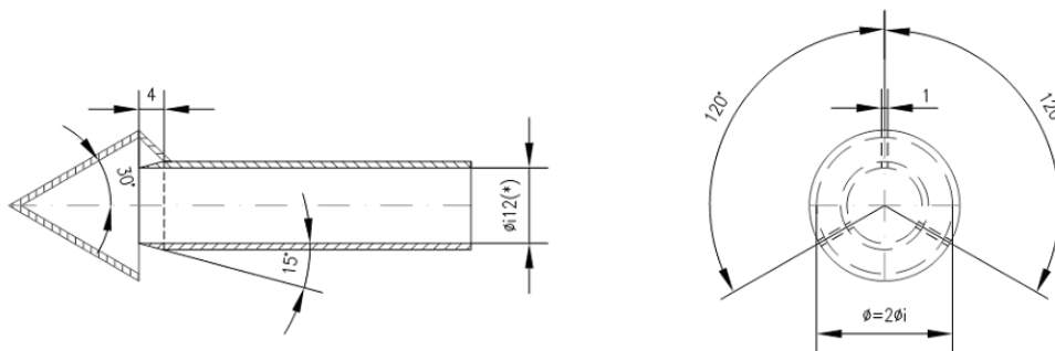
Figure A4a.App4/13 Particulate sampling probe configuration
