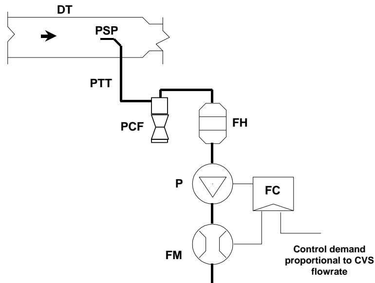
Figure A4a.App4/12 Particulate Sampling System
