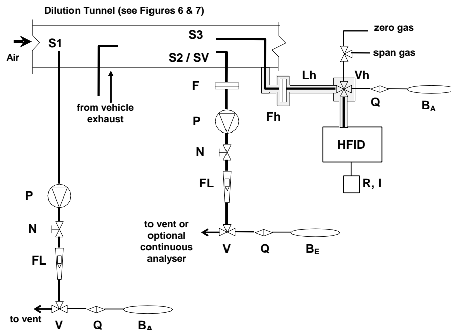
Figure A4a.App3/10 Gaseous Emissions Sampling Schematic
