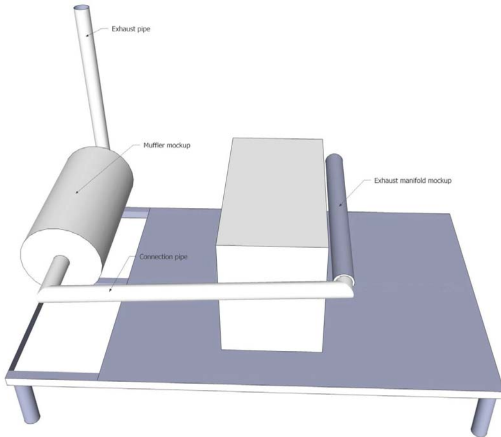
Figure 6 The exhaust system
