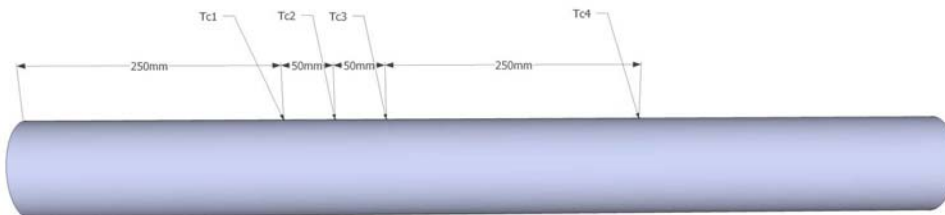
Figure 8 Thermocouples on the exhaust manifold mockup
