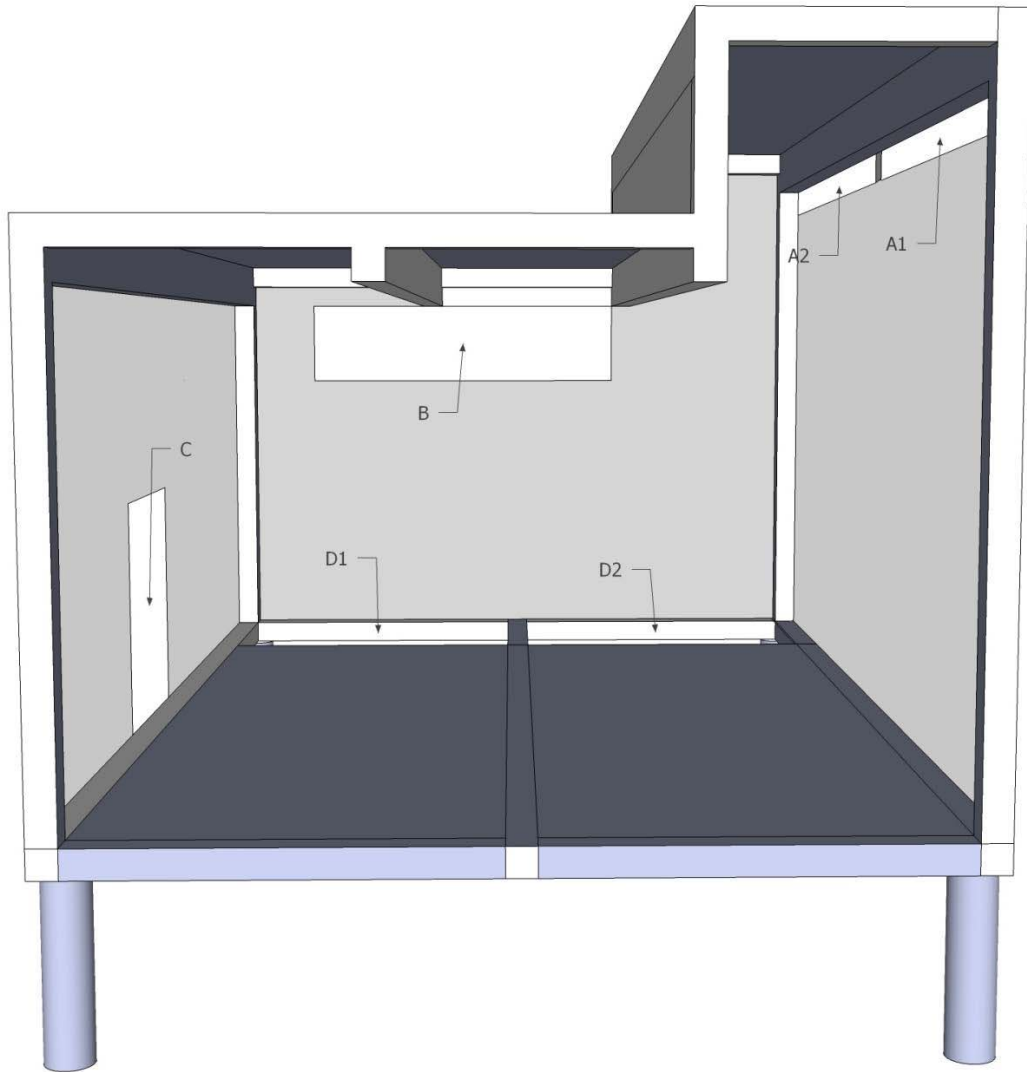
Figure 4 Apertures in the test apparatus
