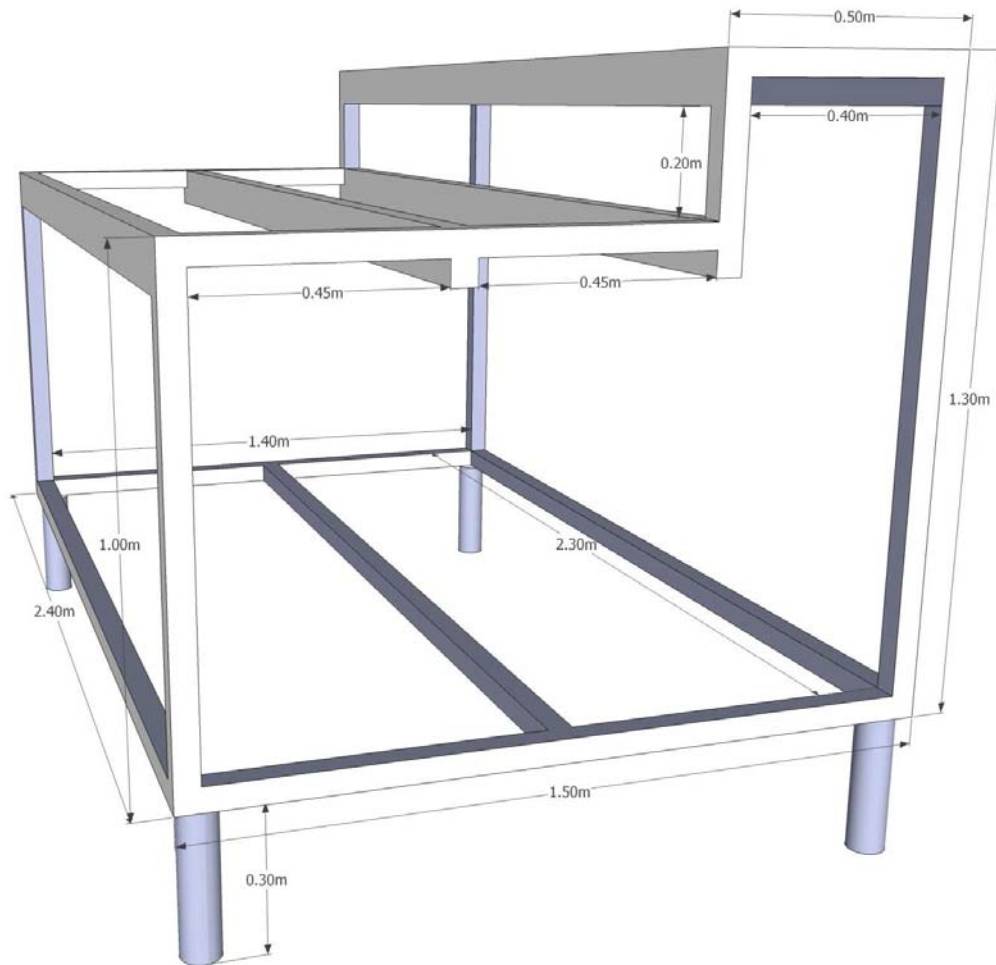
Figure 3 Framework for the test apparatus
