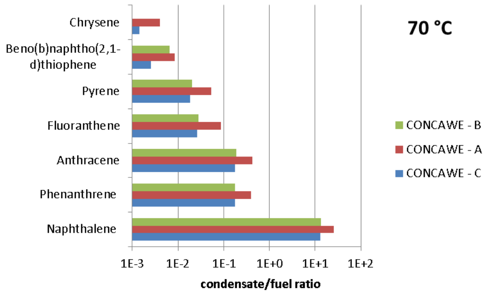
Fig. 3.11: Condensate-to-fuel ratios for selected PAHs at 70 °C
