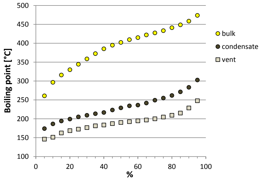
Fig. 3.6: Boiling point distributions of the bulk fuel, the condensate and the field samples (yellow).
