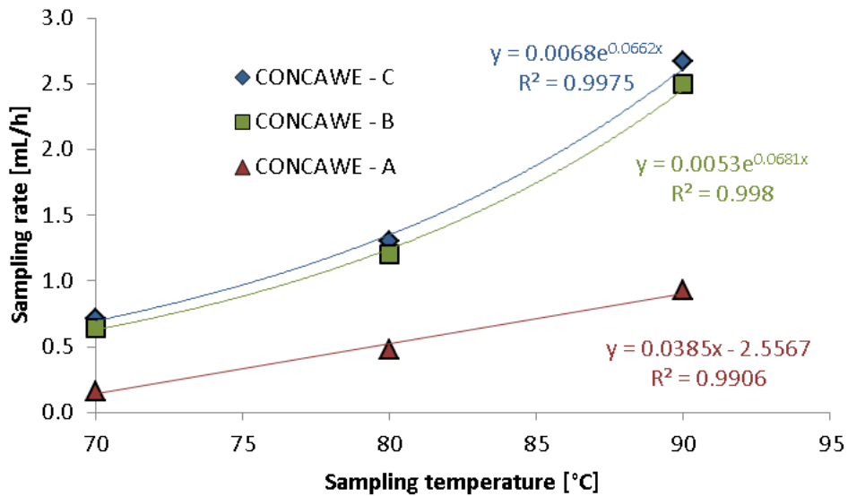
Fig. 3.14: Condensate sampling rates for CONCAWE-A, CONCAWE-B and CONCAWE-C
