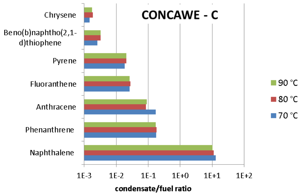
Fig. 3.10: Condensate-to-fuel ratios for selected PAHs for HFP condensate CONCAWE-C
