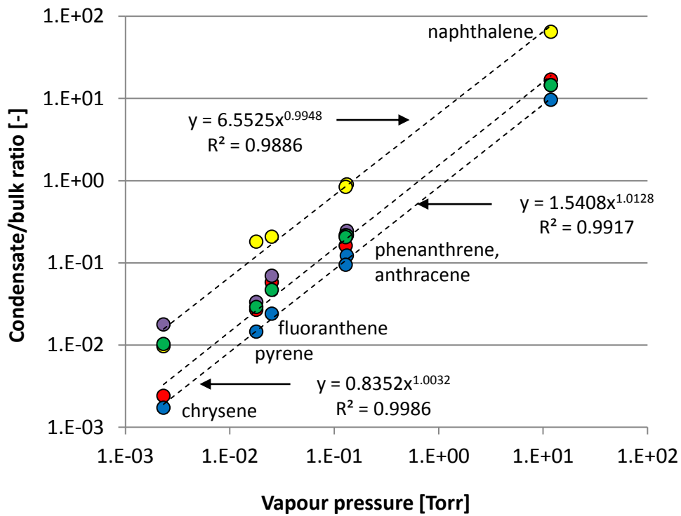
Fig. 3.10: Fume to bulk ratios of PAH mass fractions as function of the vapor pressure.
