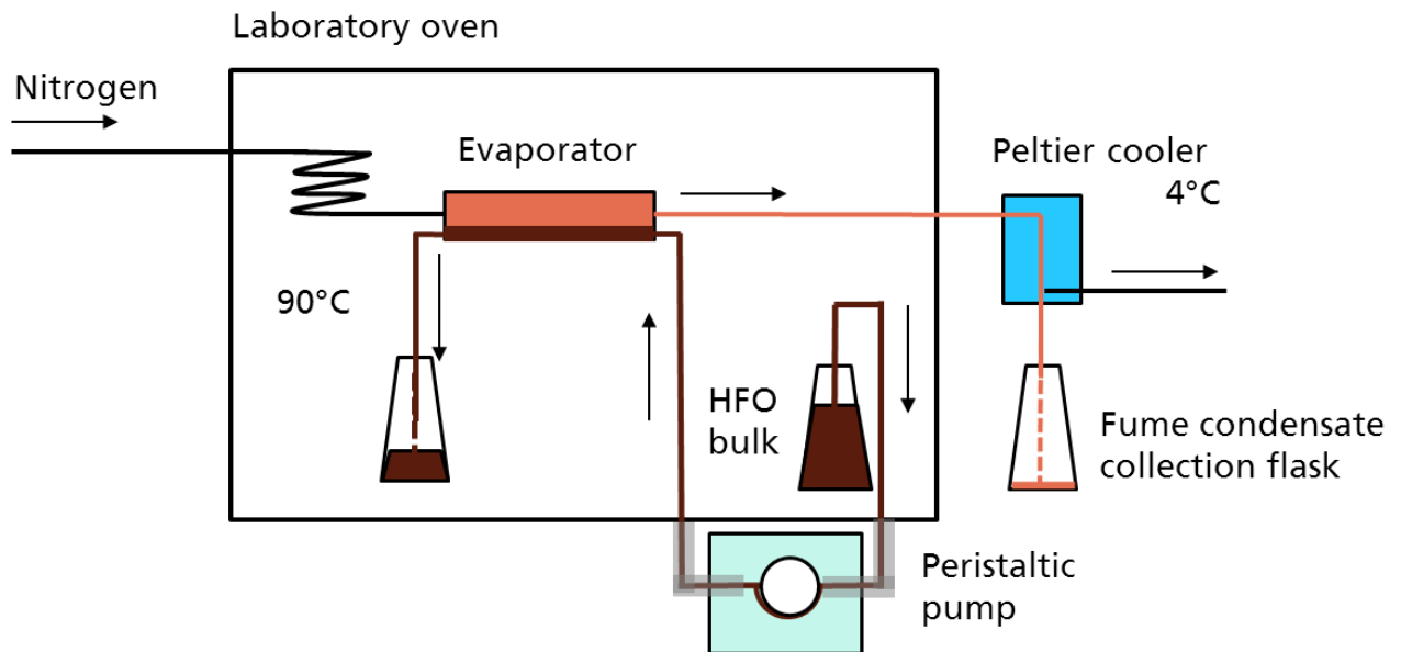
Fig. 2.1: Schematics of the laboratory set-up for fume collection at 90 °C.
