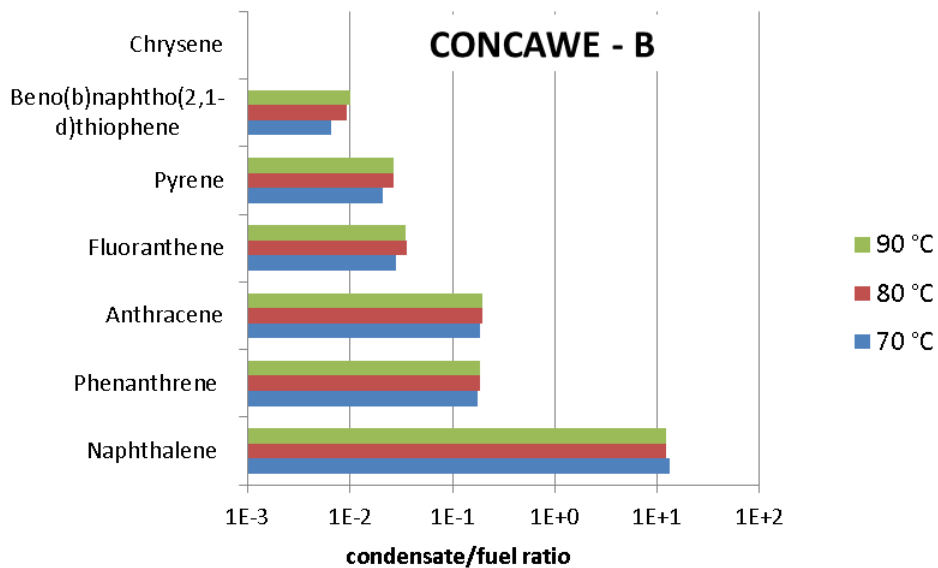
Fig. 3.9: Condensate-to-fuel ratios for selected PAHs for HFP condensate CONCAWE-B
