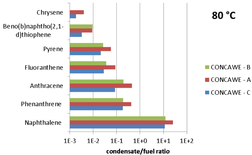
Fig. 3.12: Condensate-to-fuel ratios for selected PAHs at 80 °C
