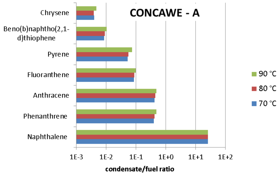
Fig. 3.8: Condensate-to-fuel ratios for selected PAHs for HFP condensate CONCAWE-A
