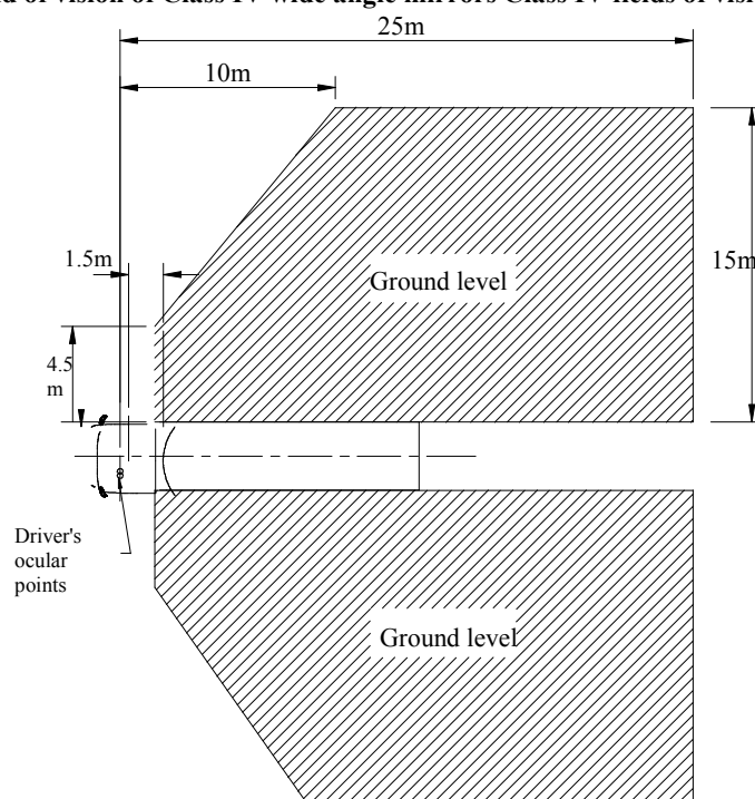
Figure 7 Field of vision of Class IV wide-angle mirrors Class IV fields of vision
