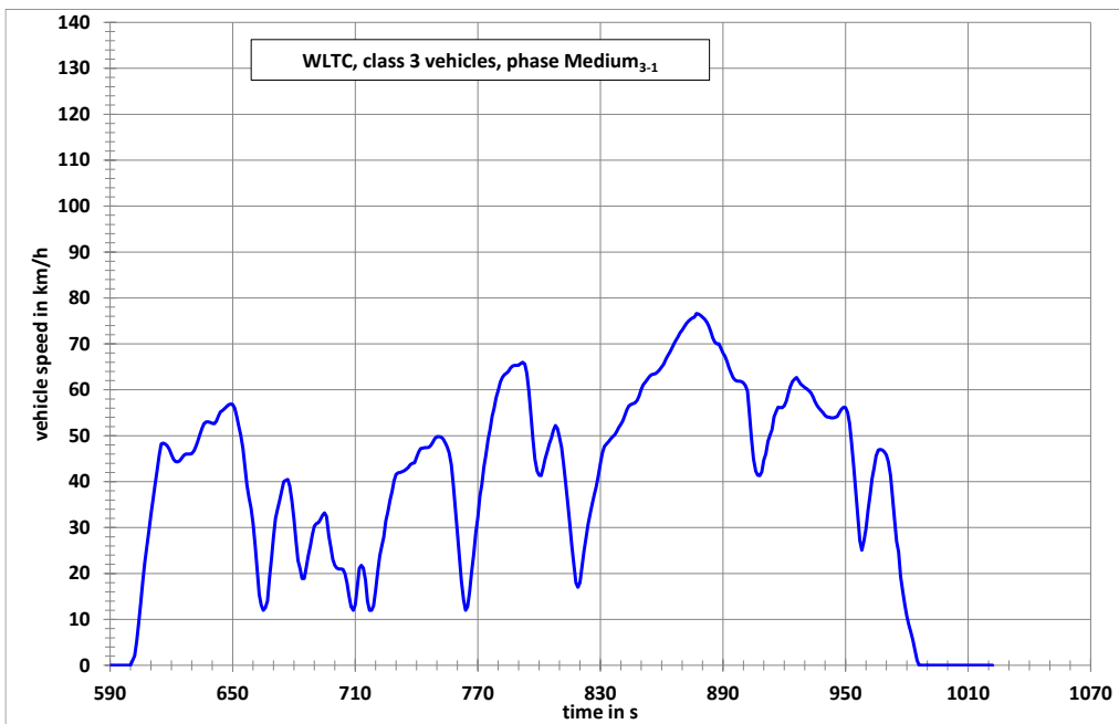
WLTC, Class 3 vehicles, phase Medium 3-1
