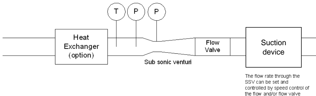
Schematic of a subsonic venturi tube (SSV)
