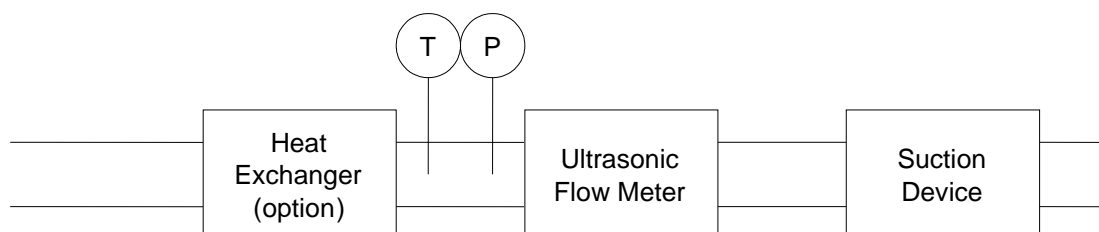
Schematic of an ultrasonic flow meter (UFM)
