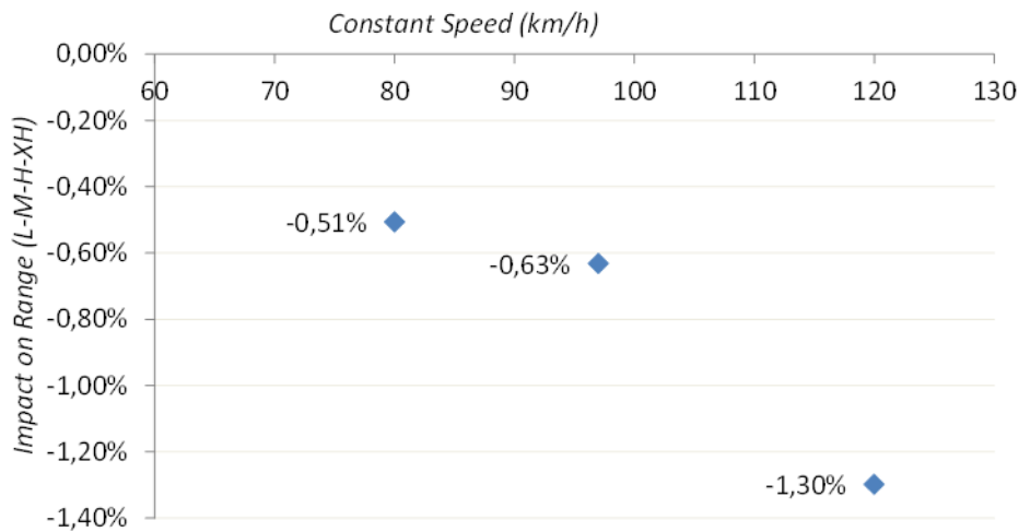
Figure 25 Validation data for shorten test procedure provided by ACEA (Renault)
