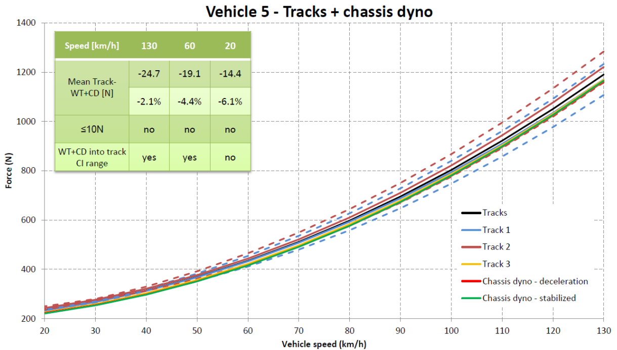
Figure 13 Comparison of road load curves for the coast down method on the tracks and the wind tunnel + chassis dyno method (deceleration and stepwise method). Dashed lines show confidence intervals for the tracks
