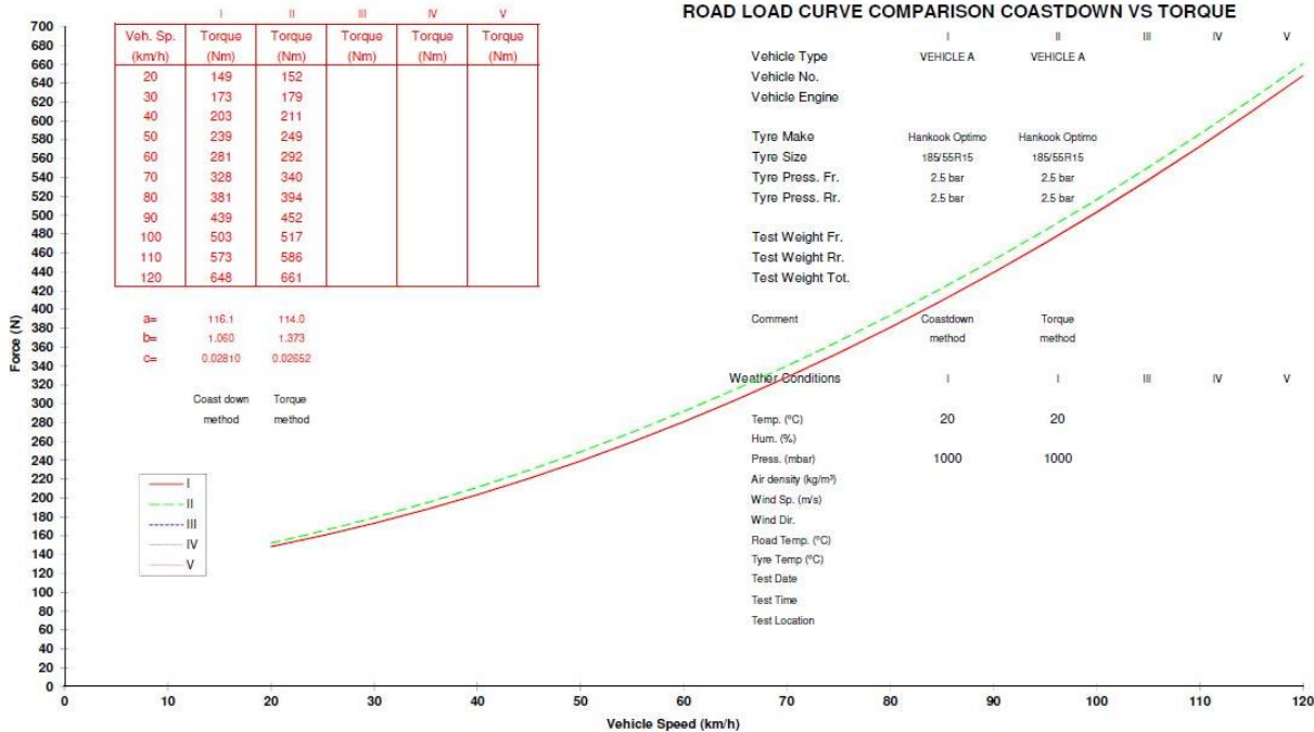
Figure 12 Validation results for the torque meter method
