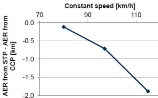
Figure 26 Validation data for shortened test procedure provided by ACEA (BMW)
