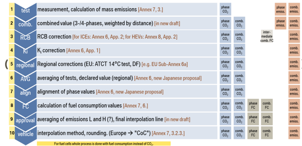
Figure 30 Post-processing scheme with the order of calculations and corrections within the UN GTR for ICE and HEV
