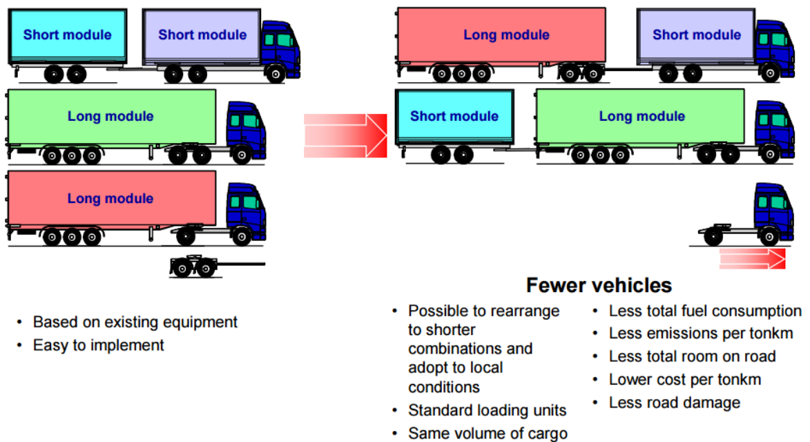
Figure. 2.11. Eurokombi concept (Source: Stefan Larsson, Director, Regulatory Projects. Weight and dimensions of heavy commercial vehicles as established by Directive 96/53/EC and the European Modular System (EMS). Workshop presentation ,June 24, 2009, Brussels)
