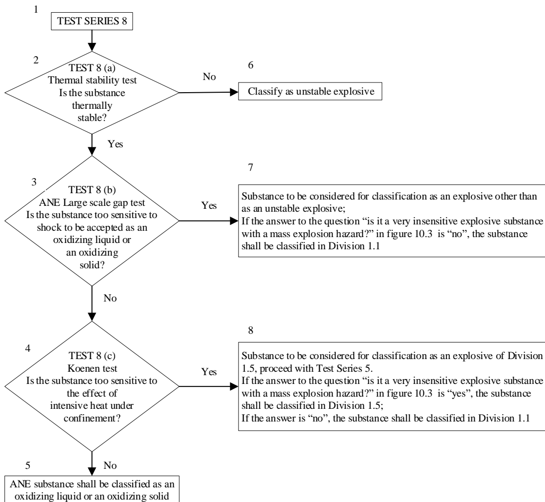
“Figure 10.4:PROCEDURE FOR AMMONIUM NITRATE EMULSION, SUSPENSION OR GEL, INTERMEDIATE FOR BLASTING EXPLOSIVES
