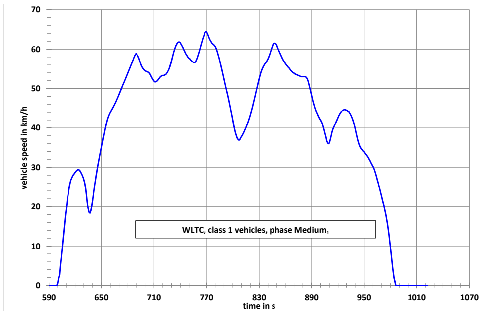
Figure A1/2 WLTC, Class 1 vehicles, phase Medium 1
