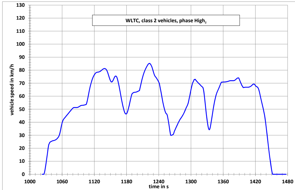
Figure A1/5 WLTC, Class 2 vehicles, phase High 2
