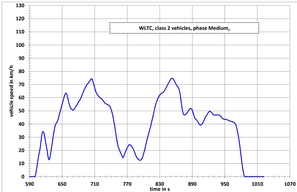
WLTC, Class 2 Vehicles, Phase Medium 2
