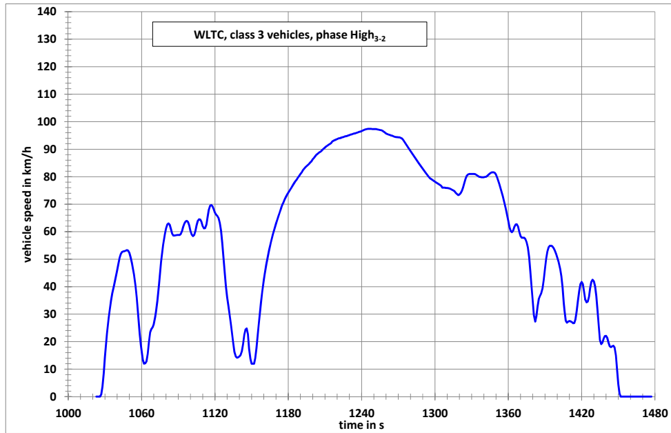
Figure A1/11 WLTC, Class 3 vehicles, phase High 3-2
