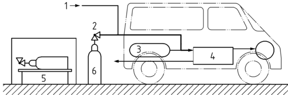
Figure A8.App7/1 Example of instrumentation
