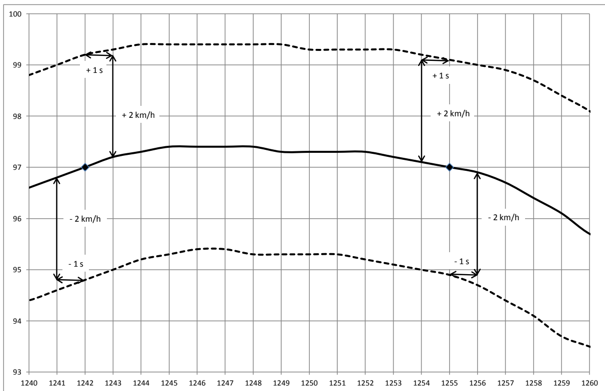
Figure A6/2 Speed trace tolerances
