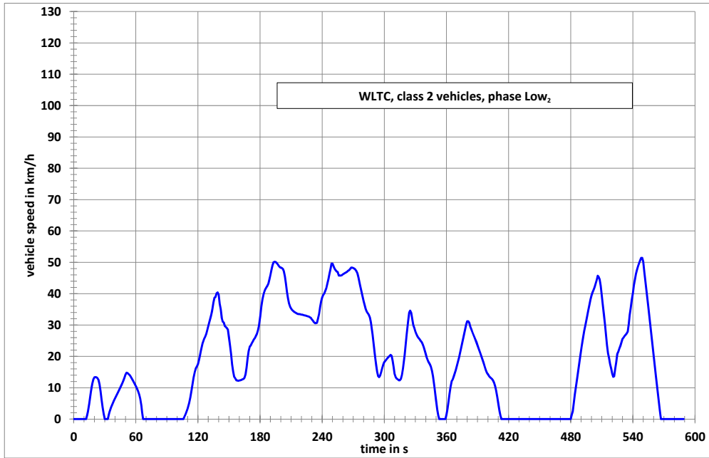
WLTC, Class 2 vehicles, phase Low 2
