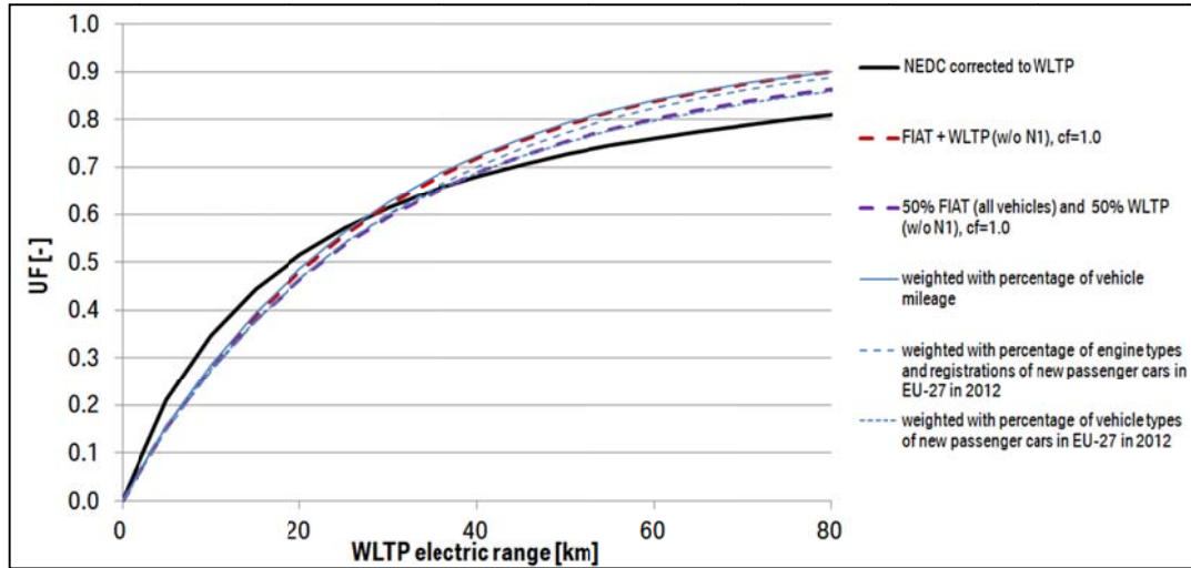
Figure 6 Comparison of different UF balancing approaches
