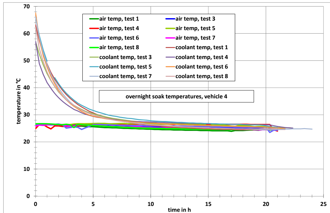
Example of overnight soak temperature monitoring
