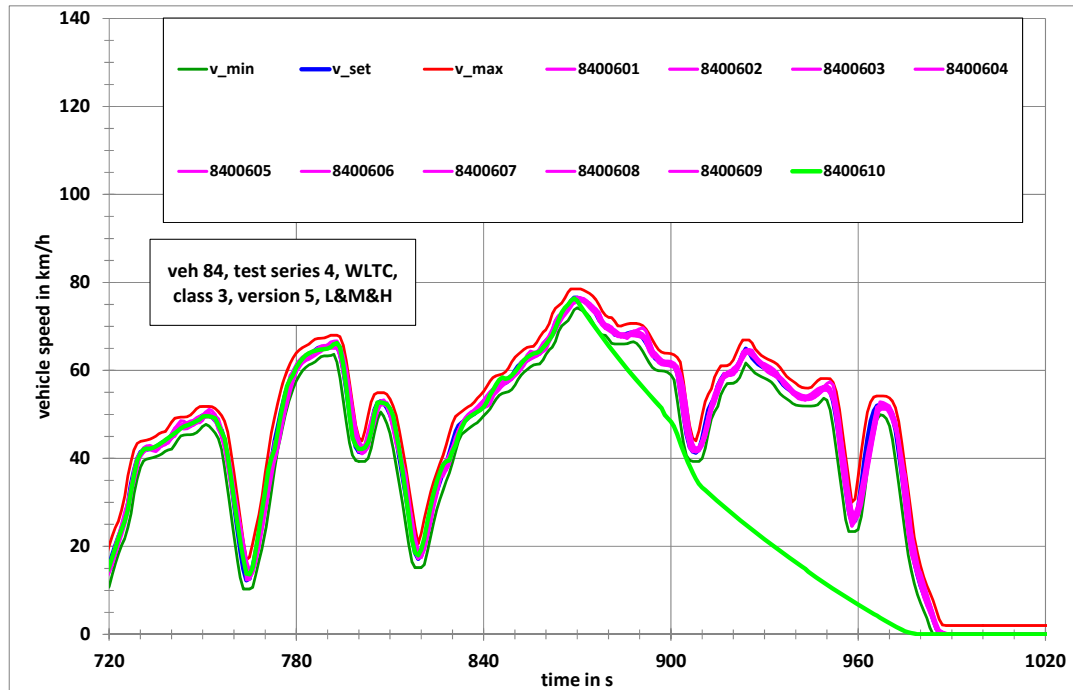
Time series of the vehicle speed for CD test 4 for vehicle 84 at break off section
