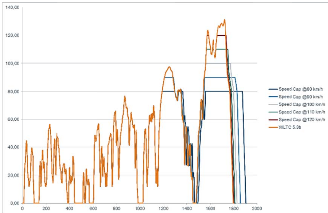
Capped speed cycle profiles for different speed caps
