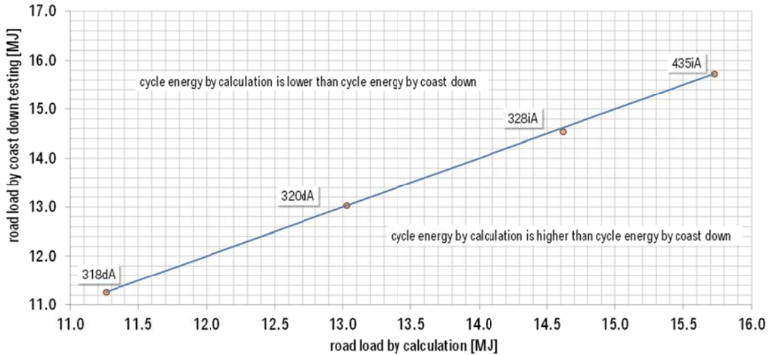
Figure 19 Results of the road load family validation tests
