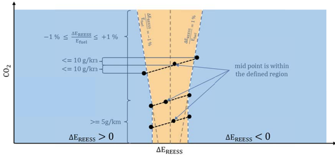
Figure 23 Graphical representation of the criteria for the second step (three tests)
