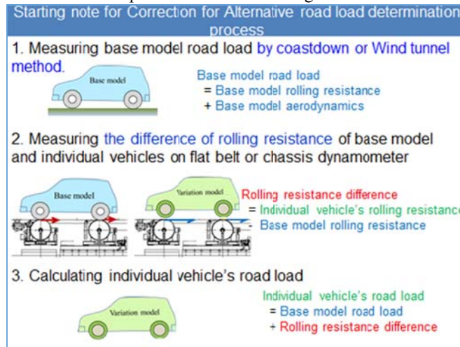
Figure 31 : Schematic representation of the three steps of the delta road load method
