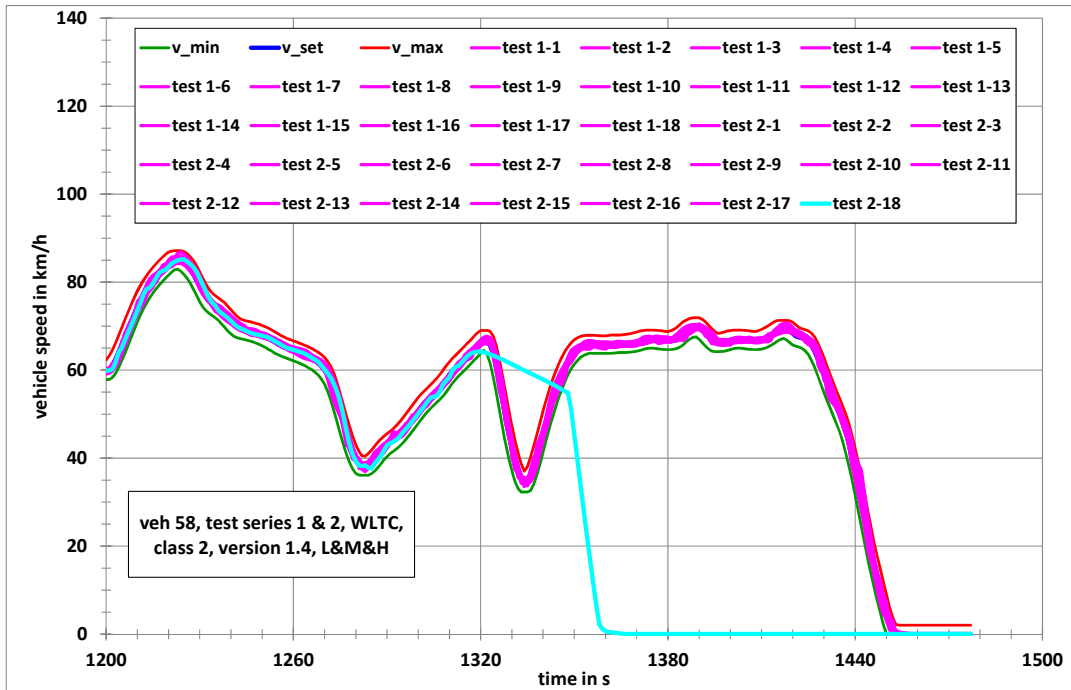
Time series of the vehicle speed for CD test 2 for vehicle 58 at break-off point
