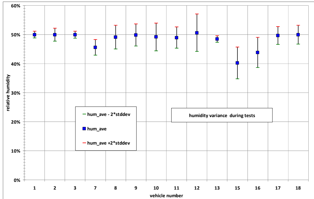
Figure 38 Test cell humidity variances during the tests
