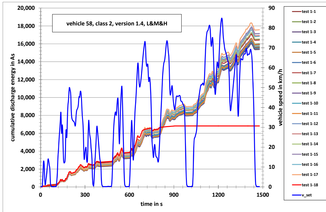
Cumulative discharge energy during the CD test 1 for vehicle 58 on the class 2 cycle (version 1.4)
