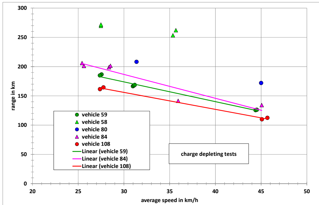
Range of the CD tests for the PEVs versus average speed of the cycles
