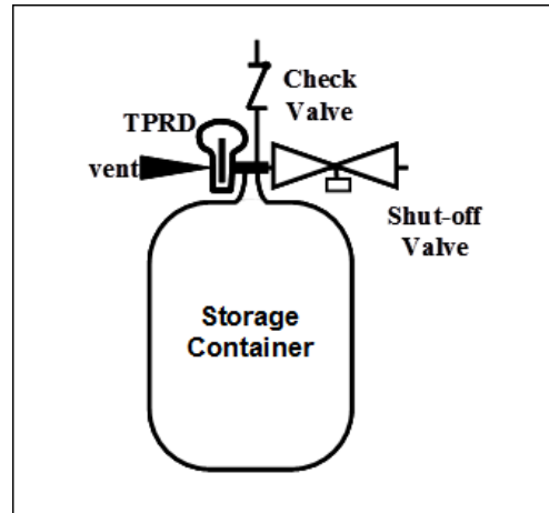
Figure 1 Typical compressed hydrogen storage system
