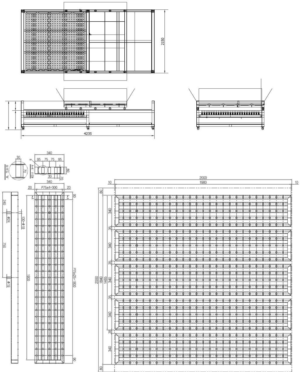
Figure 18 Illustration of KATRI LPG Burner
