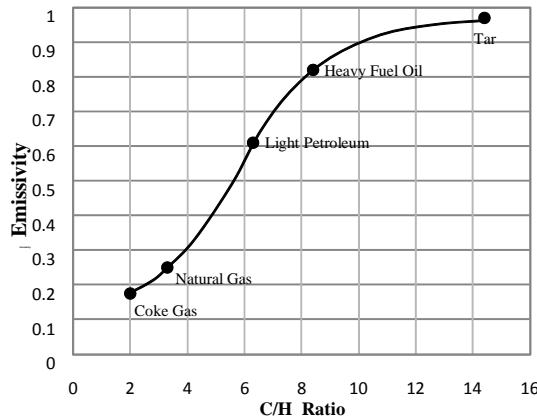
Figure 19 Emissivity of Different Fuel Flames 14
