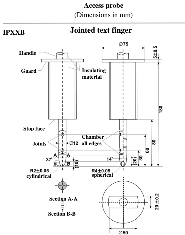
Figure 22 Jointed Test Finger
