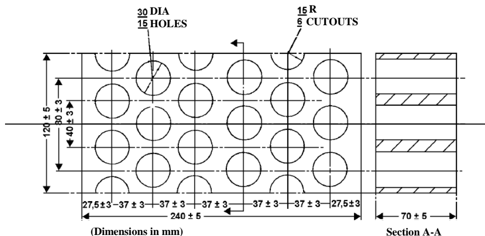
Figure 13 Dimension of Firebricks
