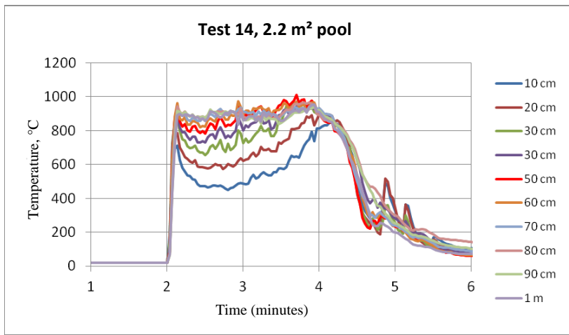
Figure 16. Temperature readings at different heights above a 2.2 m 2 pool fire
