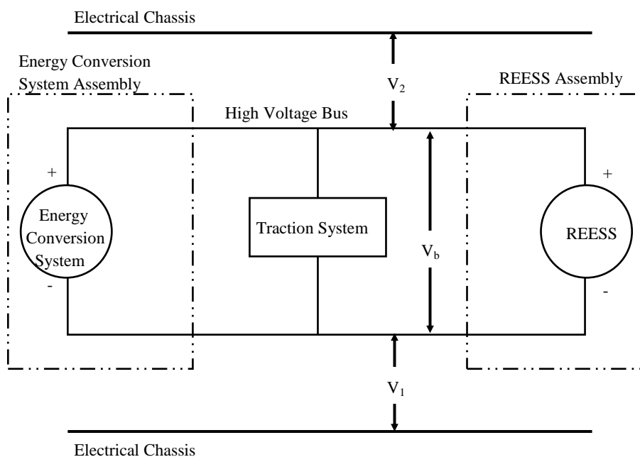
Figure 7 Measurement of V_b , V_1 , V_2
