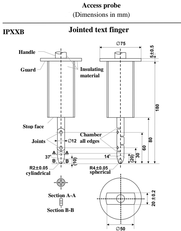
Figure 5 Jointed Test Finger
