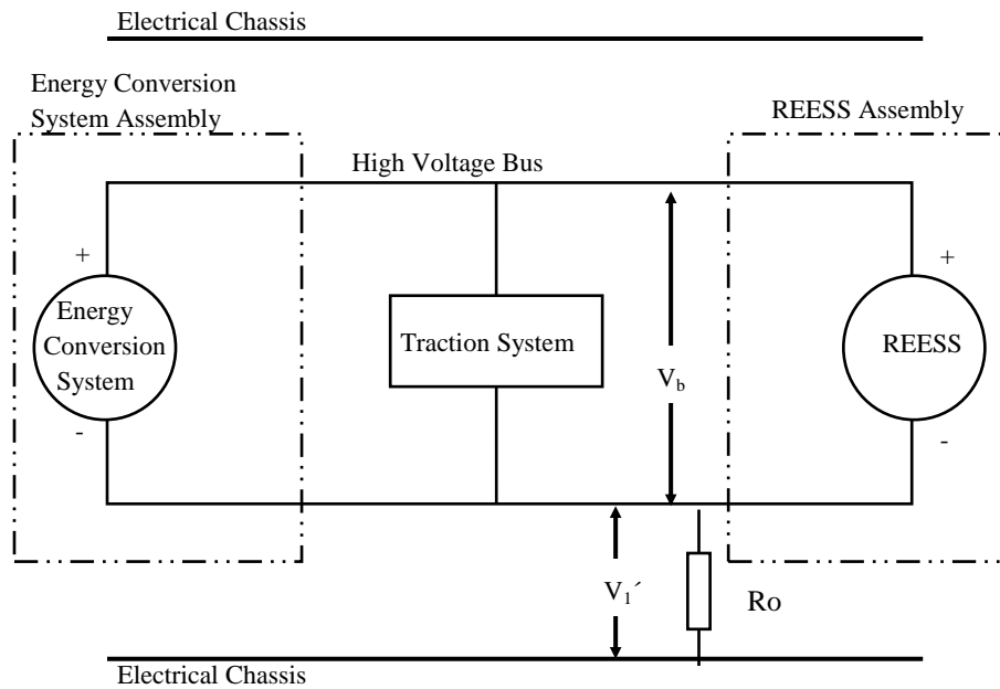
Figure 19 Measurement of V_1'
