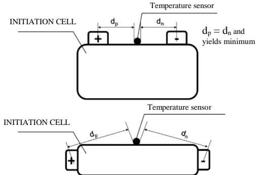
Figure 2 Example of set positions of temperature sensor in Overcharge
