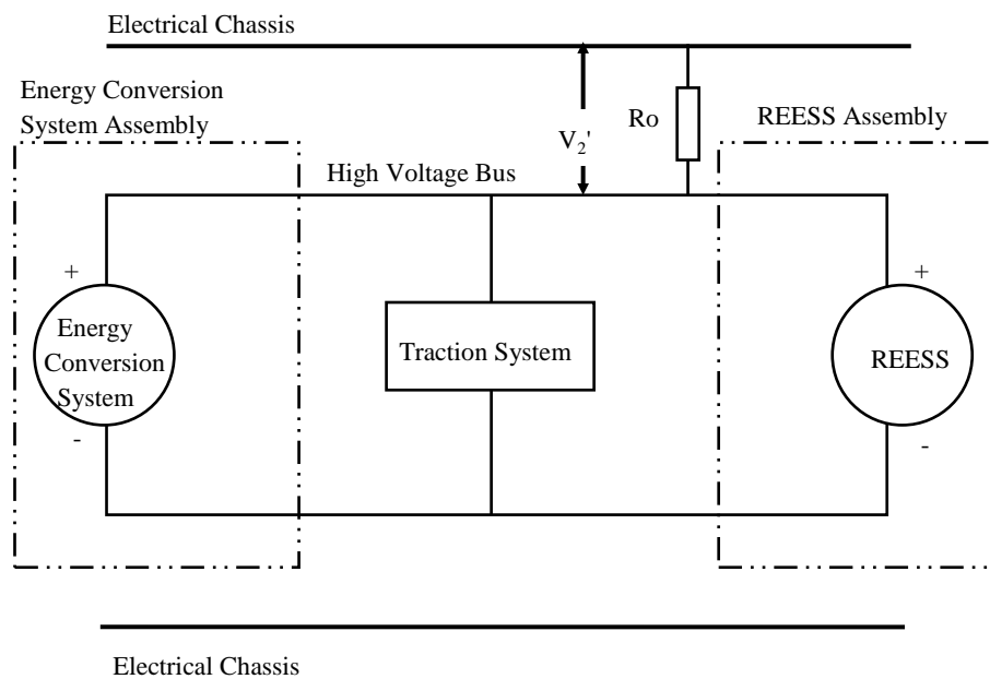
Figure 4 Measurement of V_2'
