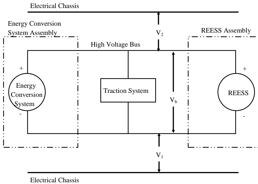
Figure 18 Measurement of V_b , V_1 , V_2
