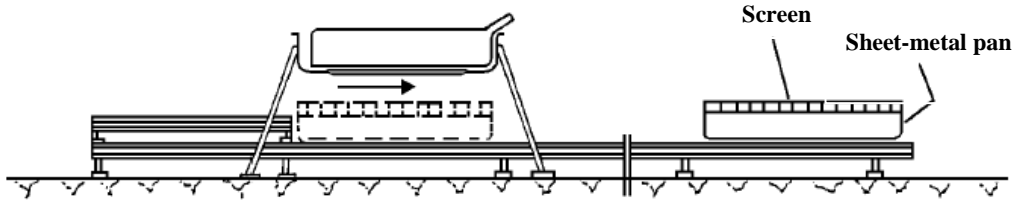
Figure 27 Phase D: End of test
