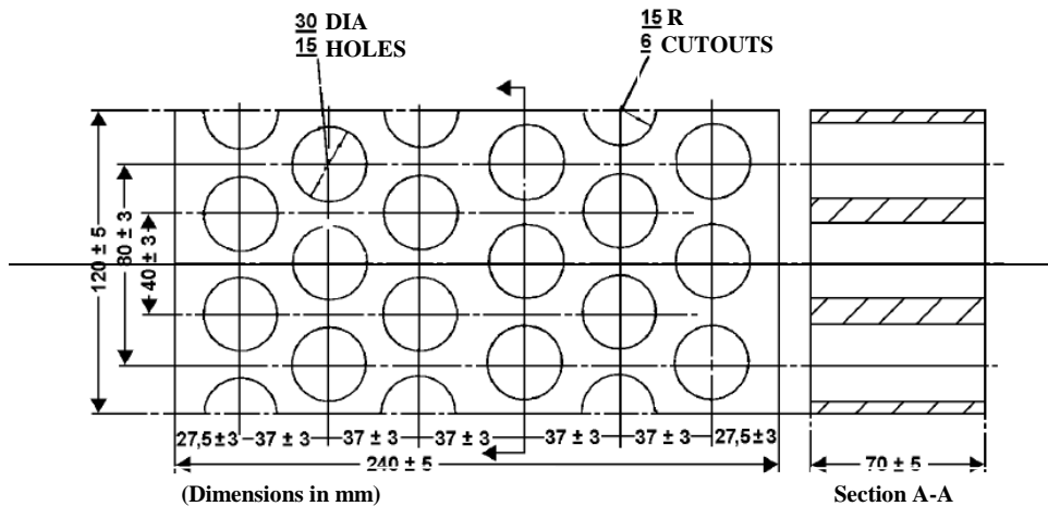
Figure 28 Dimension of Firebricks
