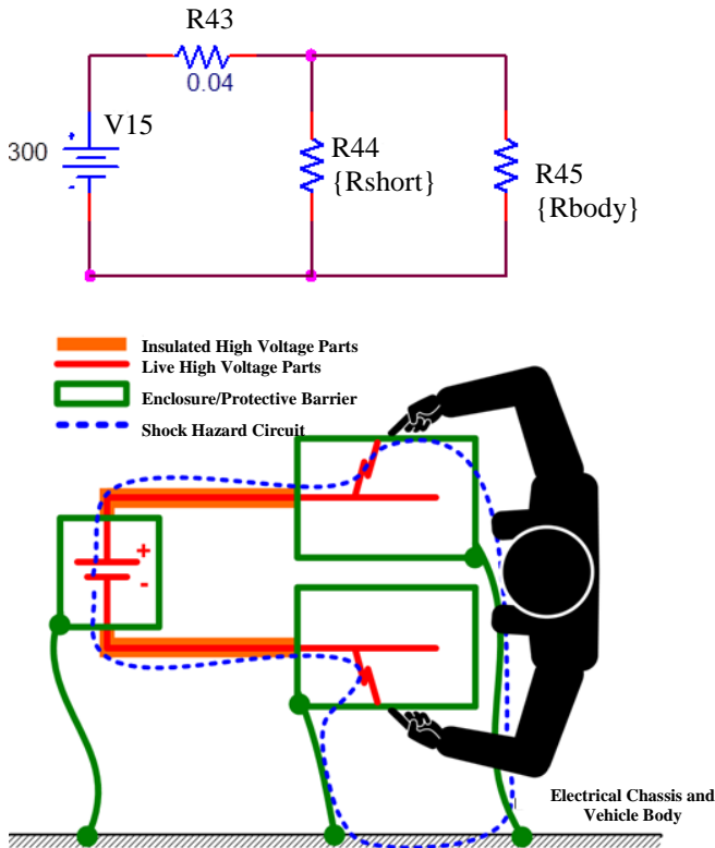
Figure 10 Potential risk scenario of indirect contact
