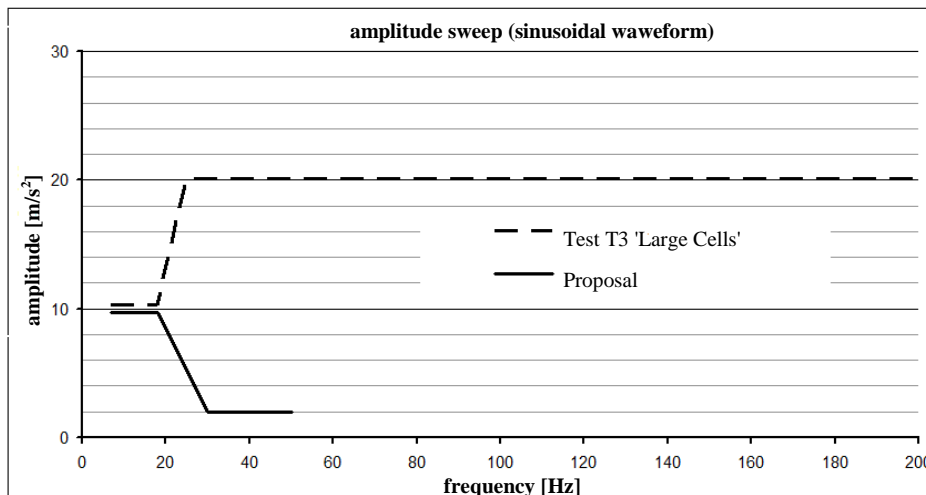
Comparison of proposed with Test T3 load curve
