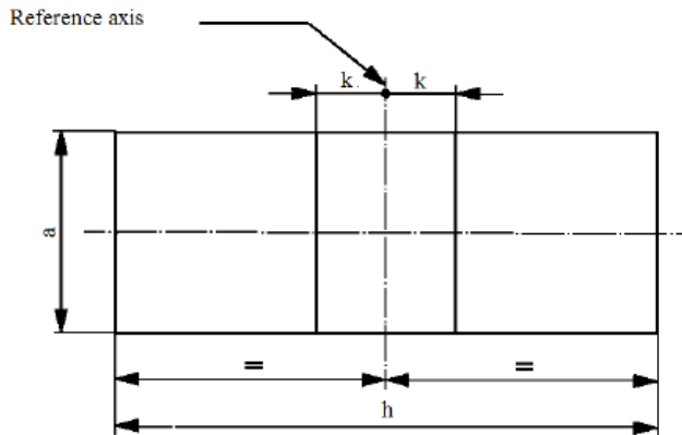
Figure 3: Front elevation of the box specification of filament light source category PY21W in Regulation No. 37
