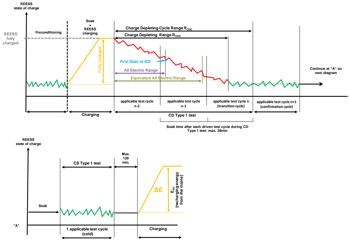
Figure A8.App1/3 OVC-HEVs, charge-depleting type 1 test with subsequent charge-sustaining Type 1 test
