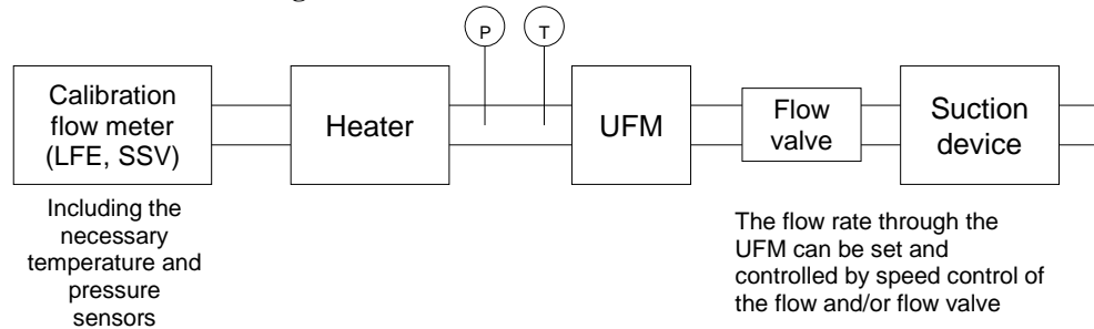
Figure A5/8 UFM calibration configuration
