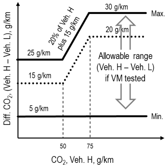
Interpolation range, electrified vehicles with Veh. M
