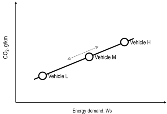
Figure A8/5 Limits for the selection of vehicle M
