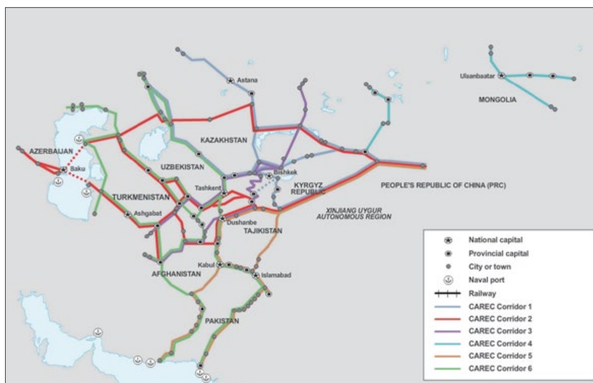
Figure 2.3 CAREC corridors
