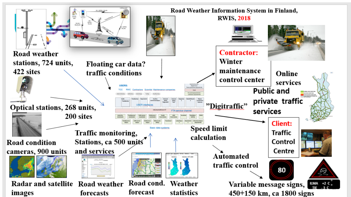
Figure II.2.5 Road weather information system in Finland
