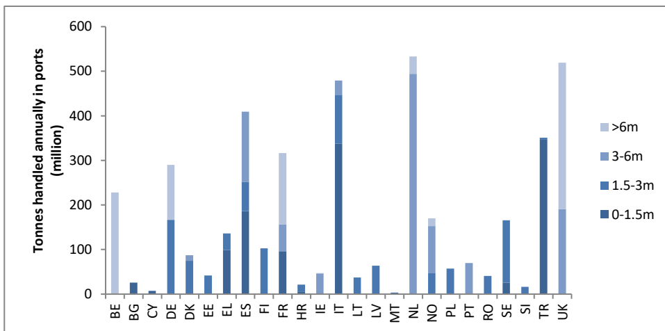
Figure I.3.39 Gross weights of cargo handled in ports affected by present-day ESL100 (based on Christodoulou et al, 2018). The different colours correspond to different ESLs as indicated by the legend.
