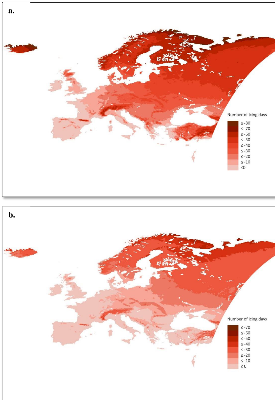
Figure I.3.7 Change in number of icing days (ID) under RCP8.5, for a) 10 th percentile values and b) 90 th percentile values
