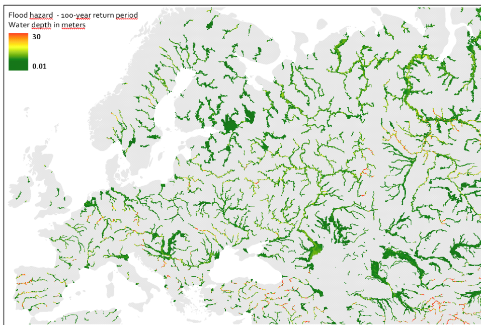
Figure I.3.36 Present flood hazard projections for the European part of the UNECE region (100-year event), data from EC-JRC
