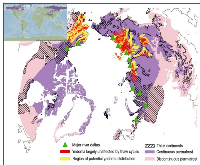
Figure I.2.5 Map of the northern circumpolar permafrost zone. Areas in yellow and red show the extent of the Yedoma permafrost (Schuur et al., 2015)
