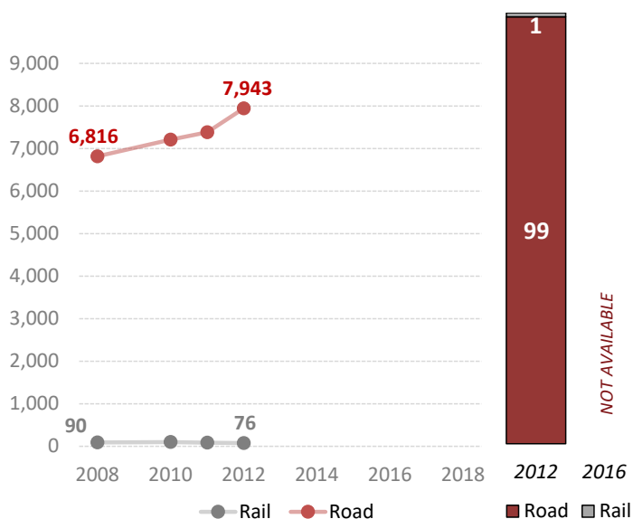
Tonne-km by mode (million) and modal share (%)
