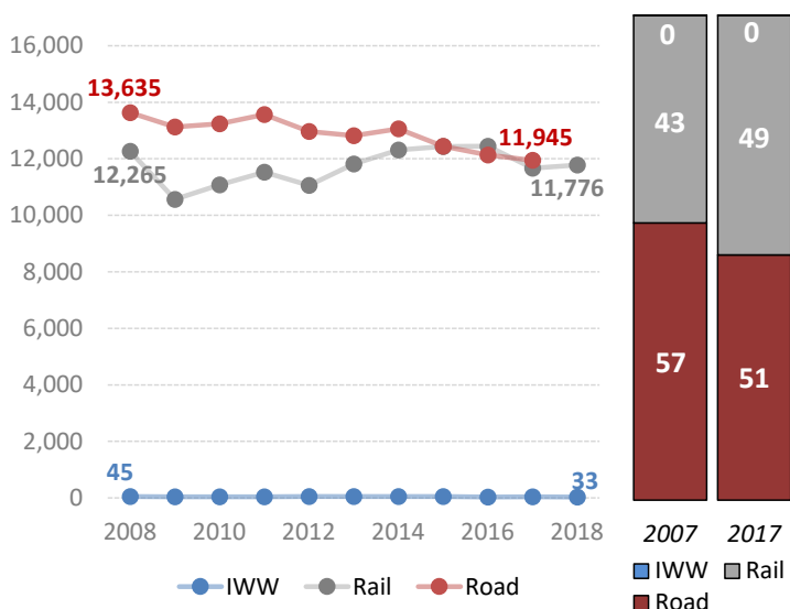
Tonne-km by mode (million) and modal share (%)
