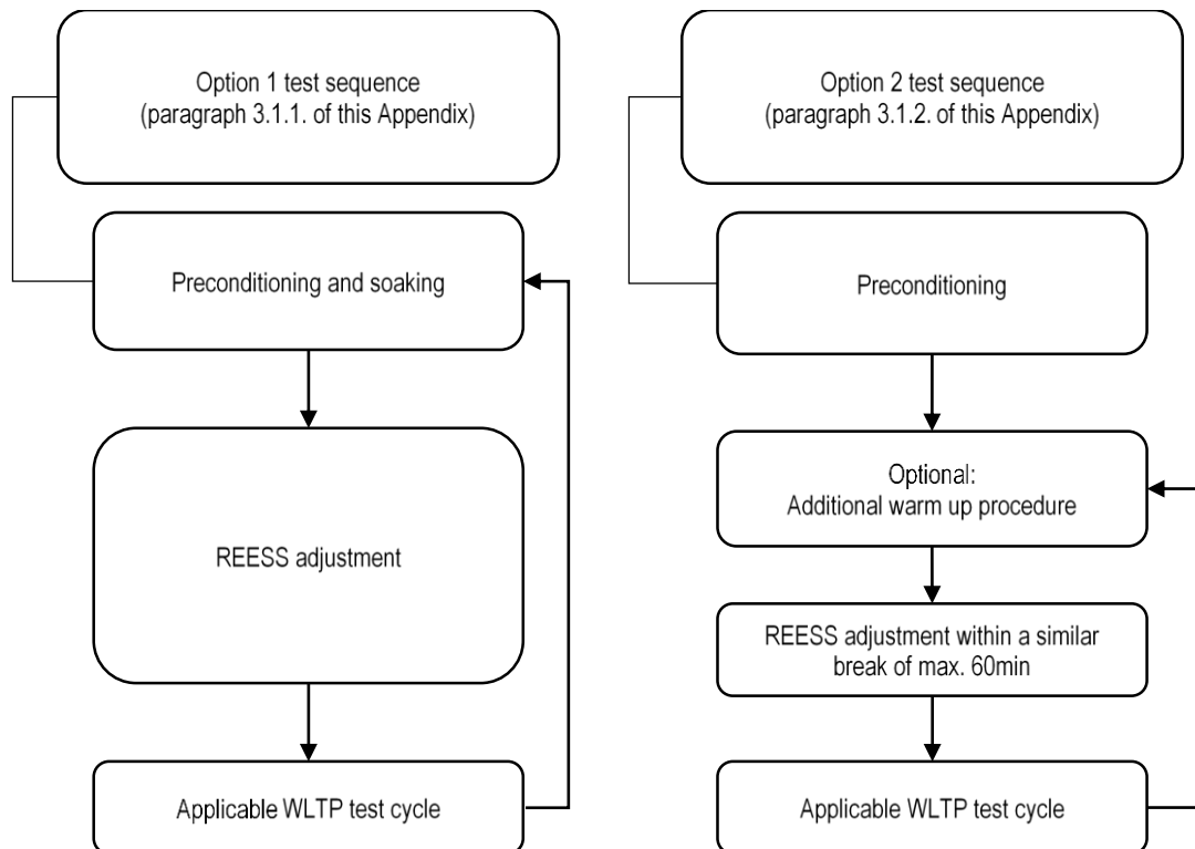
Figure A8.App2/1 OVC-HEV [and OVC-FCHV] test sequences
