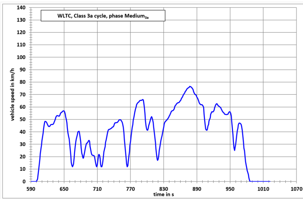
WLTC, Class 3a cycle, phase Medium 3a
