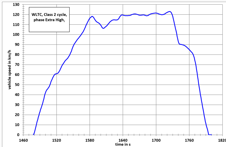
WLTC, Class 2 cycle, phase Extra High 2
