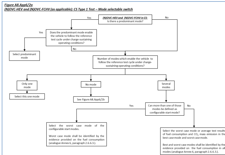
Figure A8.App6/2a and Figure A8.App6/2b Selection of a driver-selectable mode for OVC-HEVs, NOVC-HEVs [OVC-FCHVs] and NOVC-FCHVs under charge-sustaining operating condition
