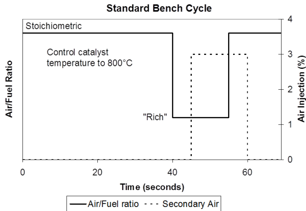
Figure C4 App1/2 Standard Bench Cycle
