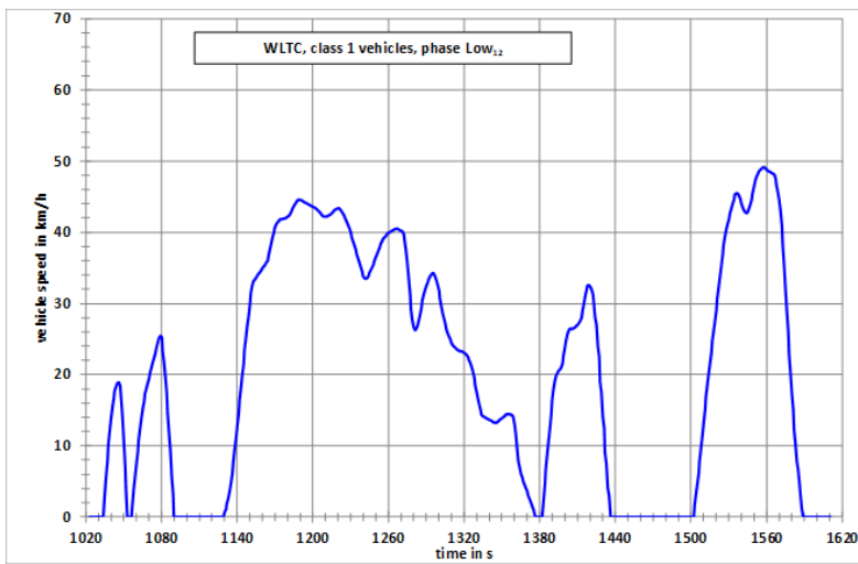
Figure A1/2b WLTC, Class 1 cycle, phase Low 12
