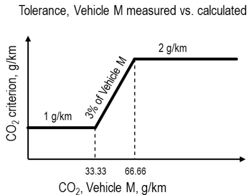
Figure A6/5 Linearity criterion for vehicle M
