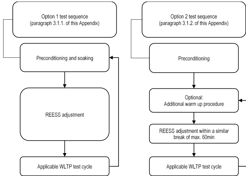
Figure A8.App2/1 OVC-HEV [and OVC-FCHV] test sequences
