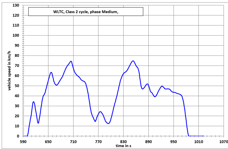
WLTC, Class 2 cycle, phase Medium 2
