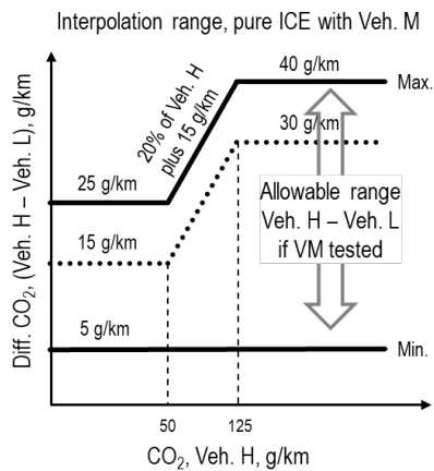
Figure A6/3 Interpolation range for pure ICE vehicles with vehicle M
