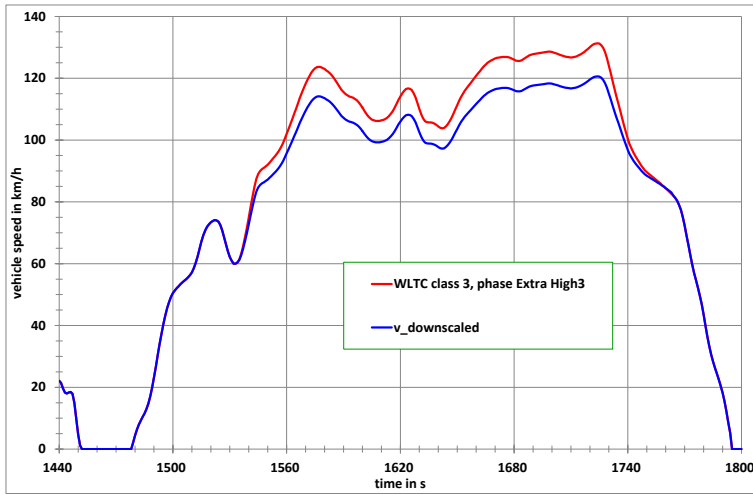
Figure A1/16 Downscaled extra high speed phase of the Class 3 WLTC
