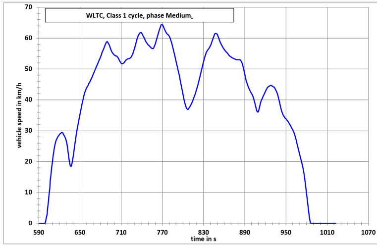
Figure A1/2a WLTC, Class 1 cycle, phase Medium 1
