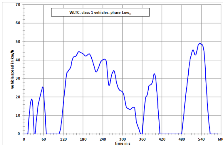
Figure A1/1 WLTC, Class 1 cycle, phase Low 11
