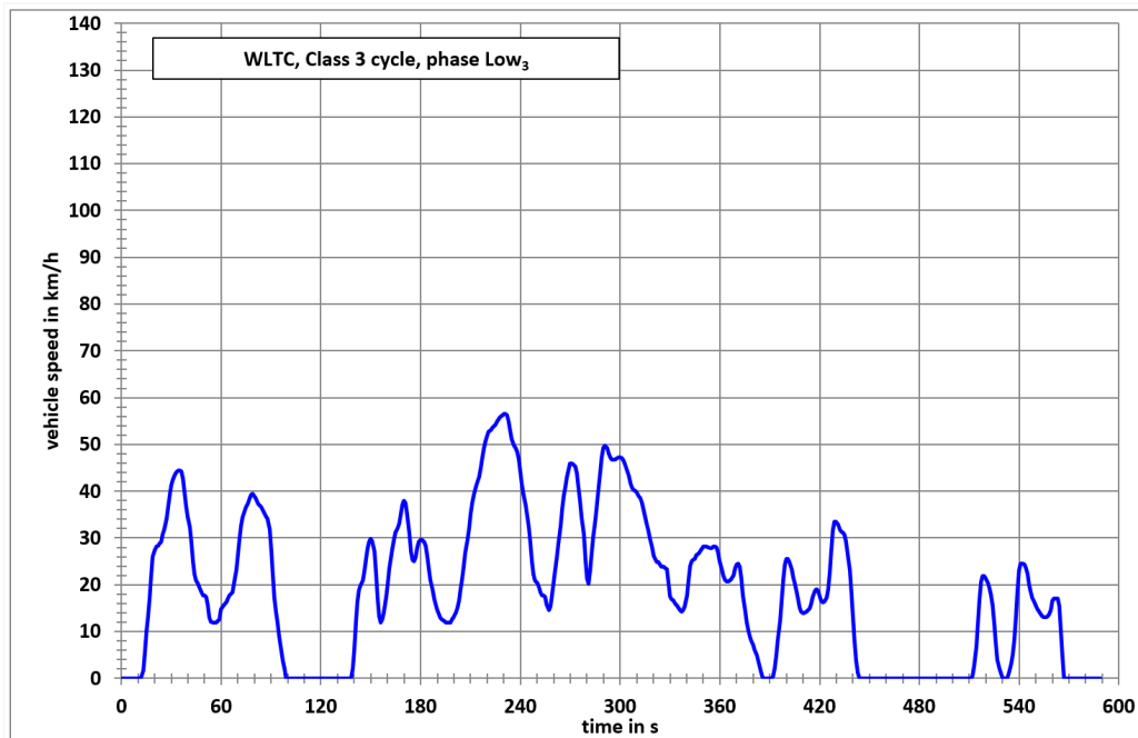
Figure A1/7 WLTC, Class 3 cycle, phase Low 3
