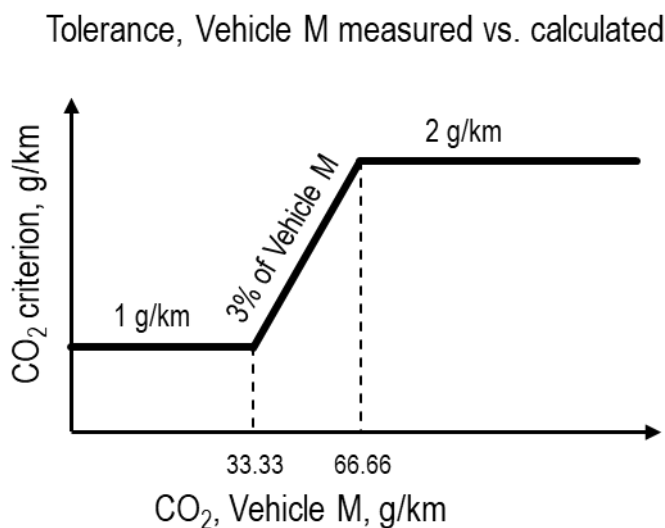
Figure A6/5 Linearity criterion for vehicle M
