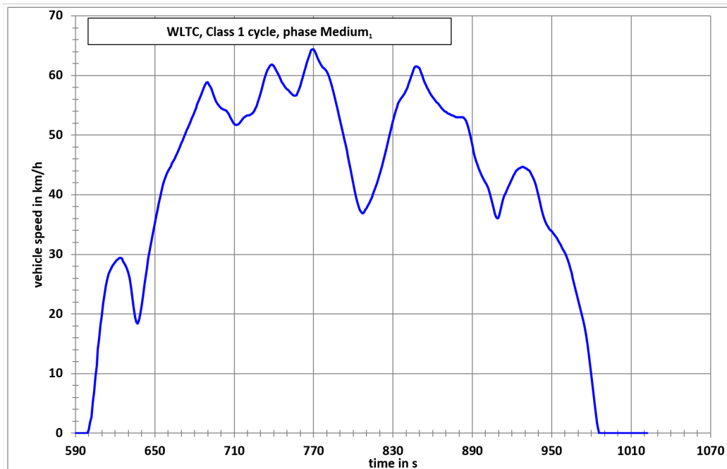
WLTC, Class 1 cycle, phase Medium 1
