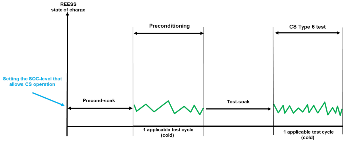
Figure A13.SA1.App1/7 NOVC-HEVs charge-sustaining Type 6 test
