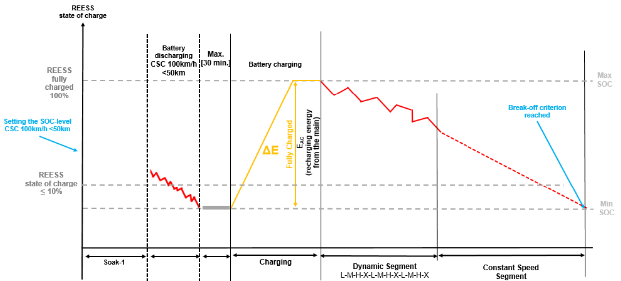
Figure A13.SA1.App1/8 PEV Type 6 test sequence
