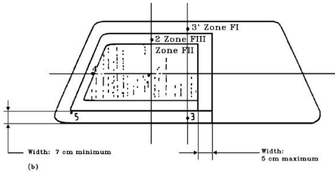
Figure 2 Prescribed points of impact for windscreens
