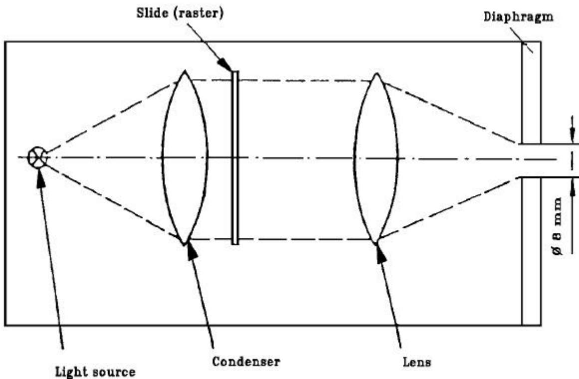
Figure 7 Optical Arrangement of the Projector
