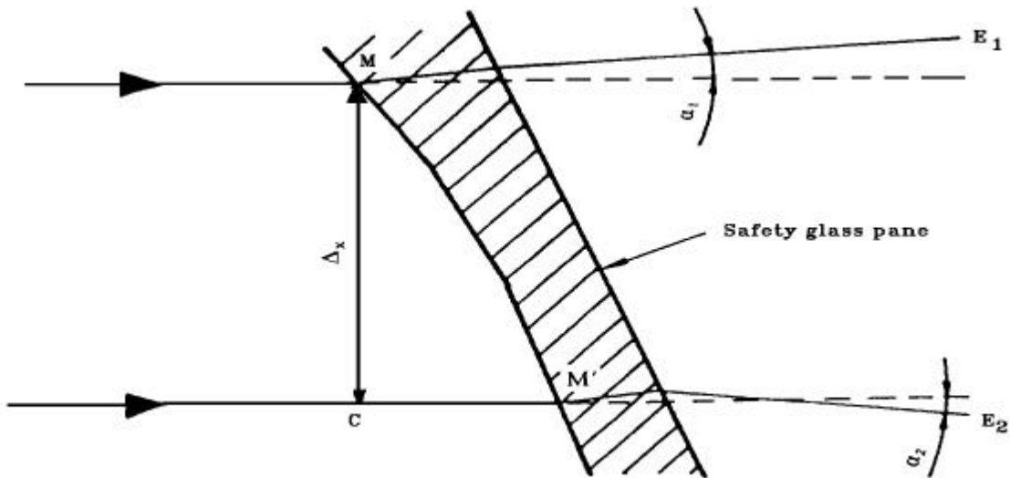
Figure 6 Diagrammatic Representation of Optical Distortion
