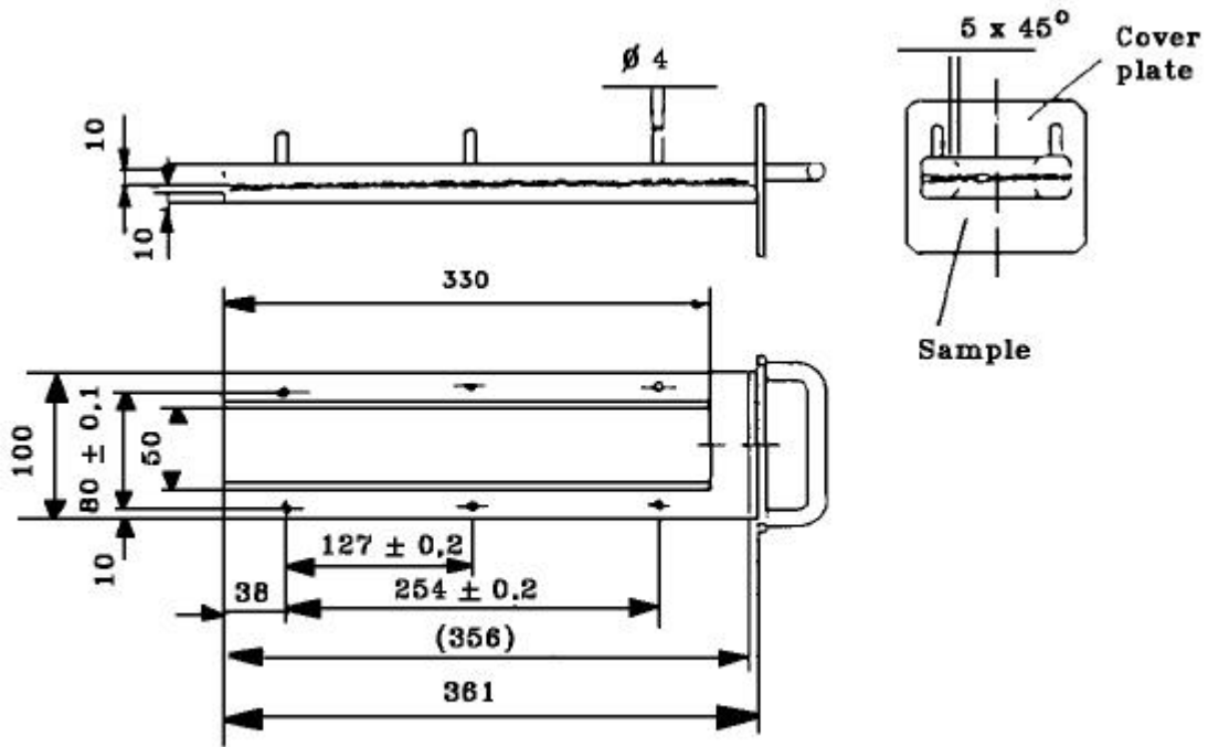
Figure 18 Example of sample holder
