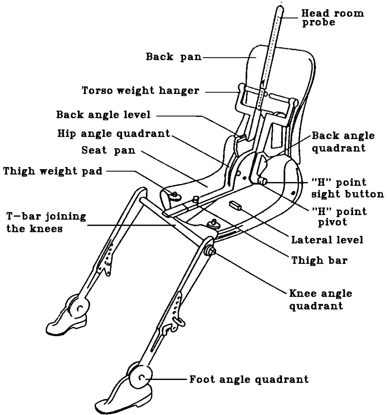
Figure 1 Designation of 3 DH machine components
