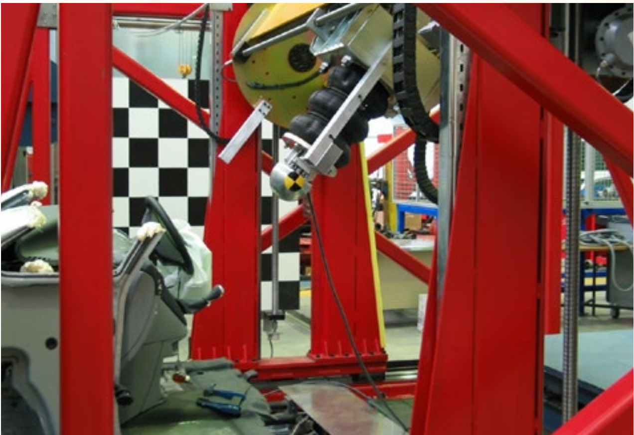
Testing machine for head impact © INTA - Spain
