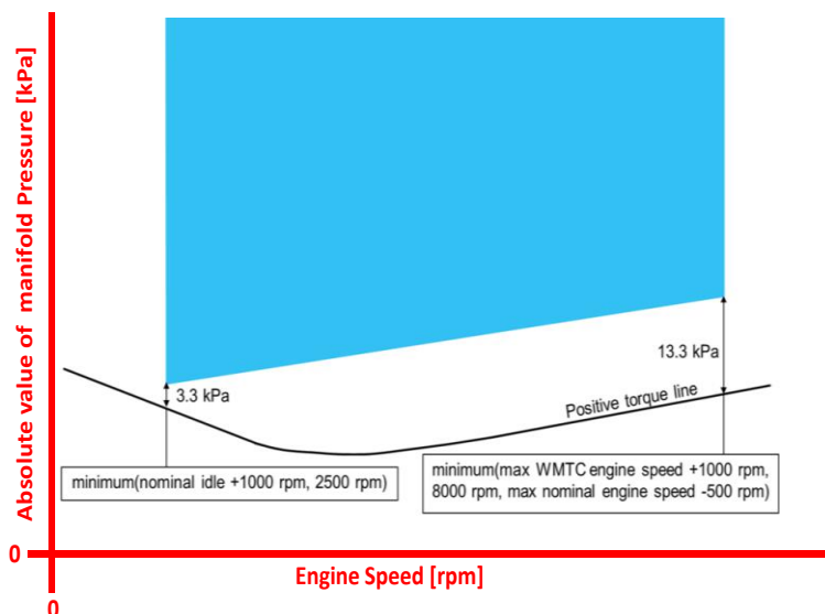
Figure 1 Operating region for misfire detection
