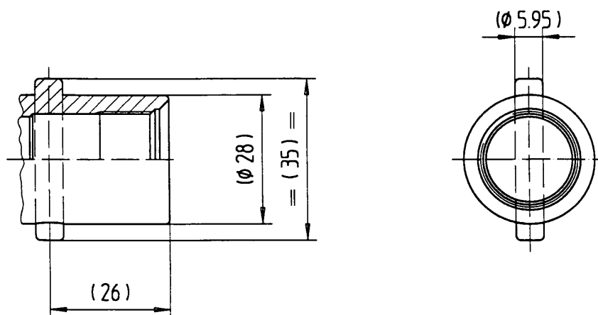
Figure 1 Connecting area of the bayonet filling unit
