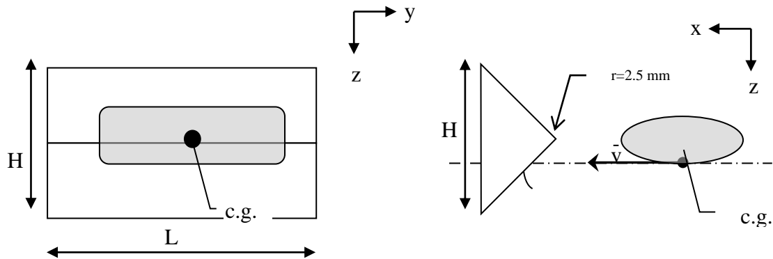
Figure 1 Description of the impact test procedure
