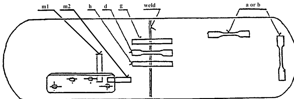
Figure 2a Containers with circumferential welds only and side-mounted valve blocks; location of test-pieces
