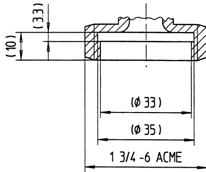
Figure 4 Connecting area of the ACME filling unit
