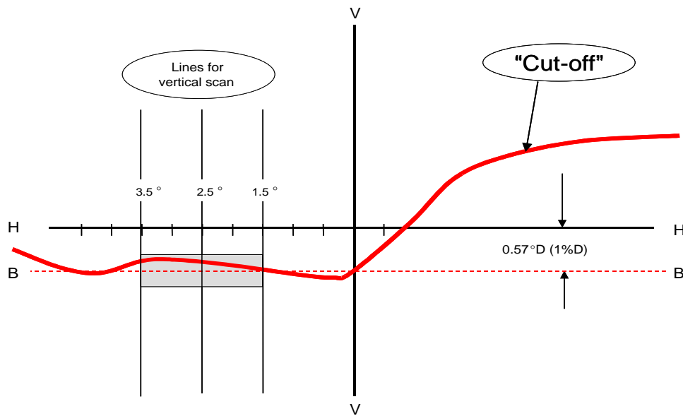
Figure 1 Measurement of "cut-off" quality
