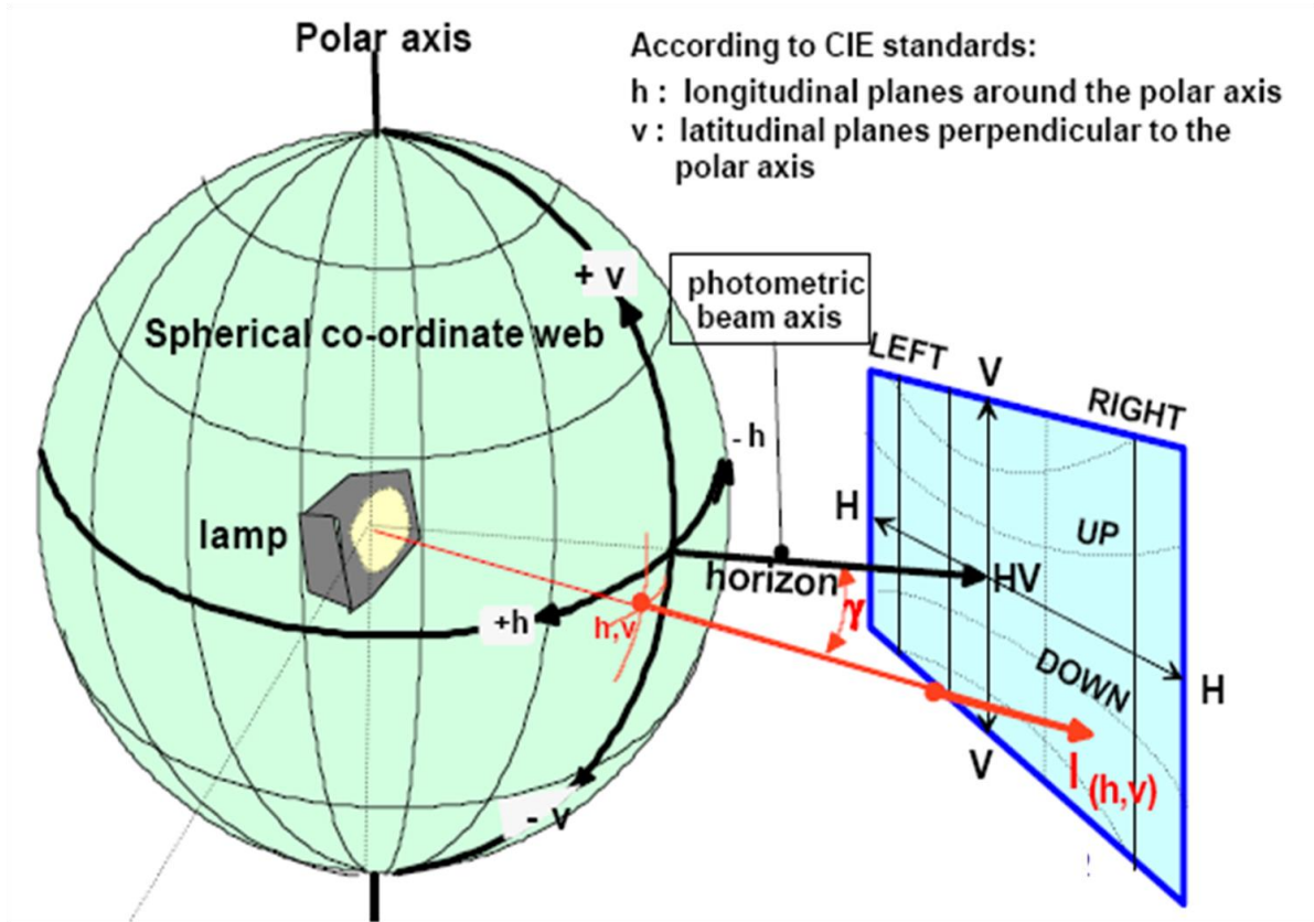
Figure A Spherical coordinate measuring system
