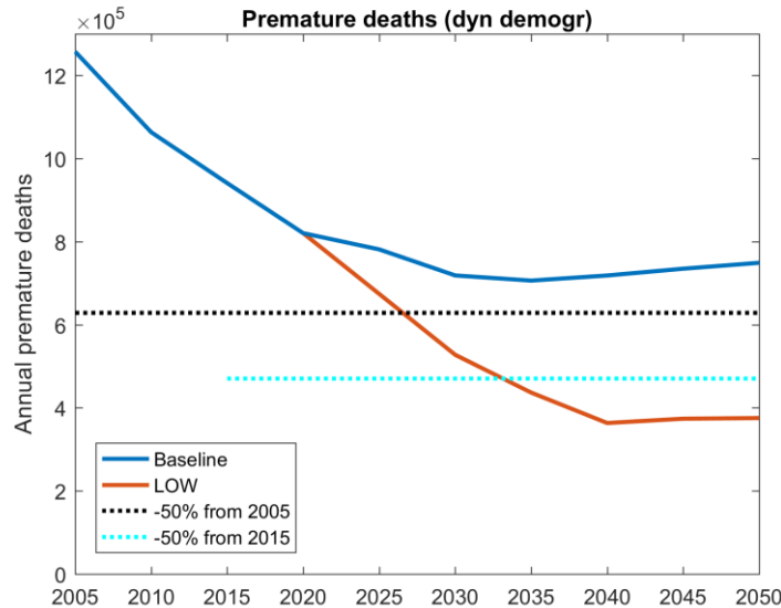
Figure 5: Absolute numbers of annual premature deaths due to PM2.5 exposure in the UNECE-region (incl. North America)
