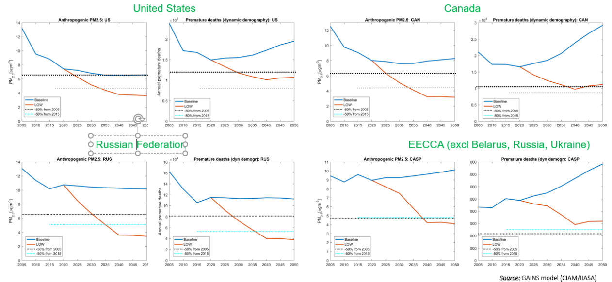
Figure A.2: Change in PM2.5 concentrations and number of premature deaths (taking into account population change and ageing – dynamic demography) for Baseline and LOW scenarios (2)
