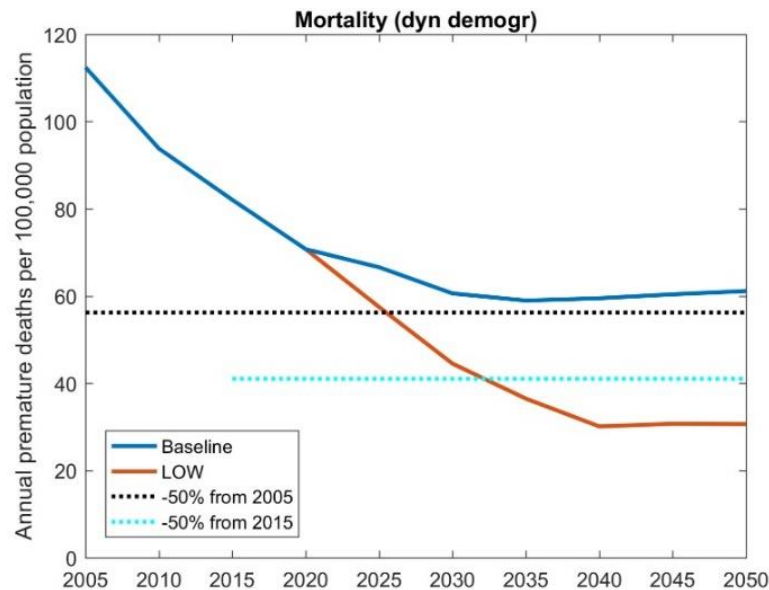
Figure 6: Mortality risk due to PM2.5 (annual premature deaths per 100.000) in the UNECE-region (incl. North America)
