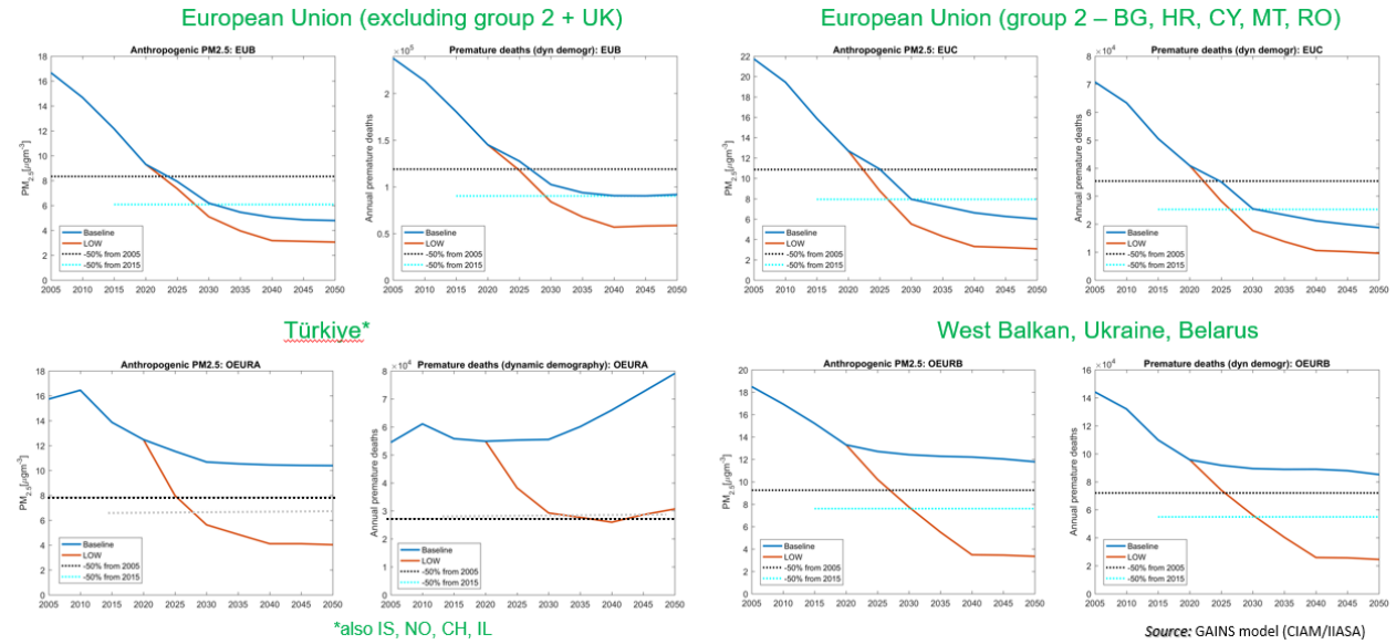
Figure A.1: Change in PM2.5 concentrations and number of premature deaths (taking into account population change and ageing – dynamic demography) for Baseline and LOW scenarios (1)
