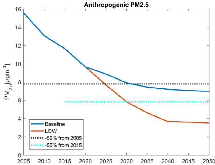
Figure 4: Average exposure to PM2.5 in the UNECE-region (incl. North America)
