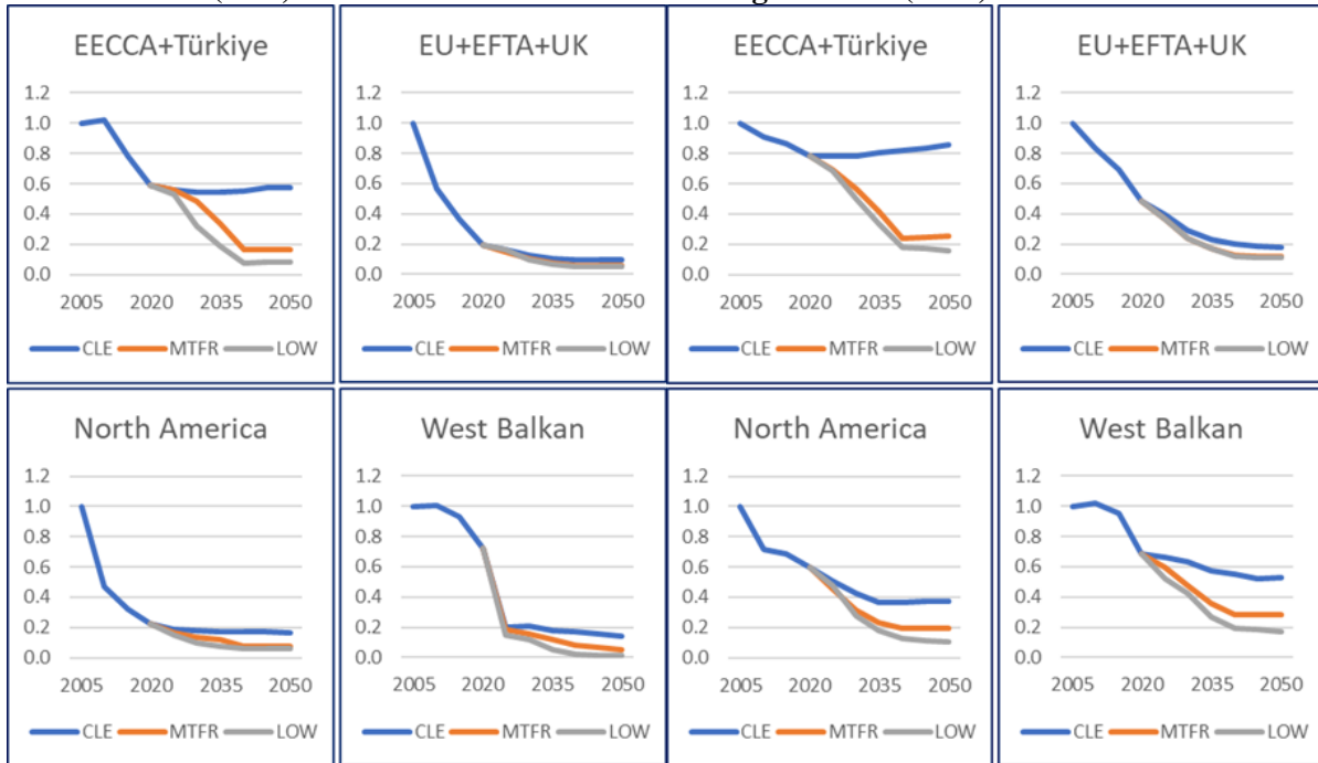
Figure 1: Emission trends in baseline (CLE), MTR and LOW scenario
