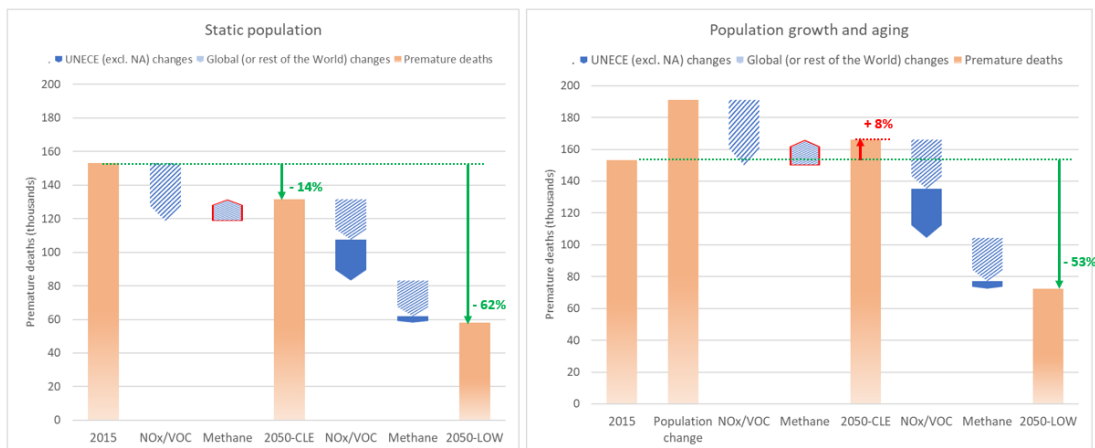
Figure 11: Reduction in annual premature deaths due to ozone exposure in the UNECE-region (excl. North America) with expected population growth (right) and without population growth (left)
