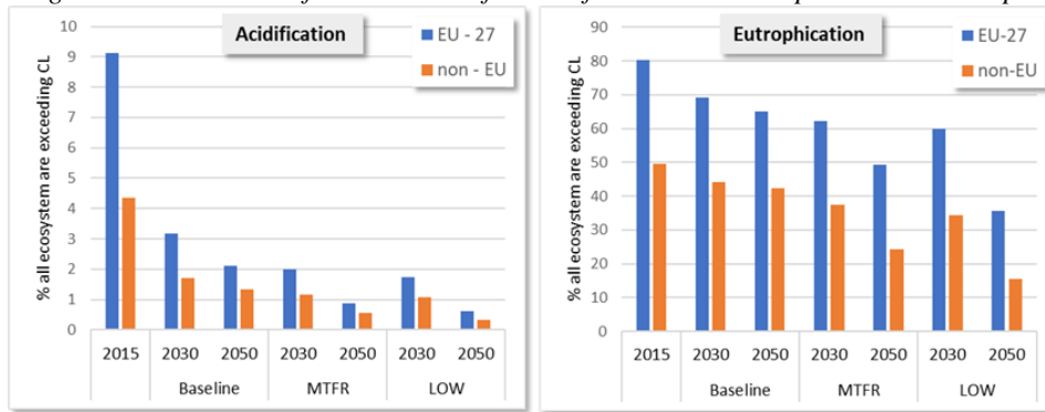
Figure 3: Exceedance of critical loads for acidification and eutrophication in Europe
