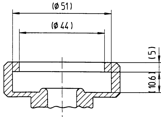
Figure 3 Connecting area of the light vehicle Euro filling unit
