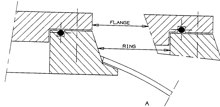
Figure 4 Examples of welded rings with flange
