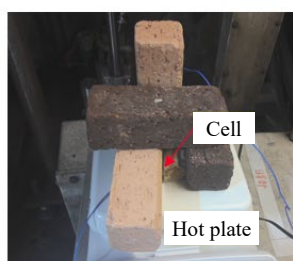
Fig. 16: Type D, high temperature heating test results (no rapid temperature rise).
