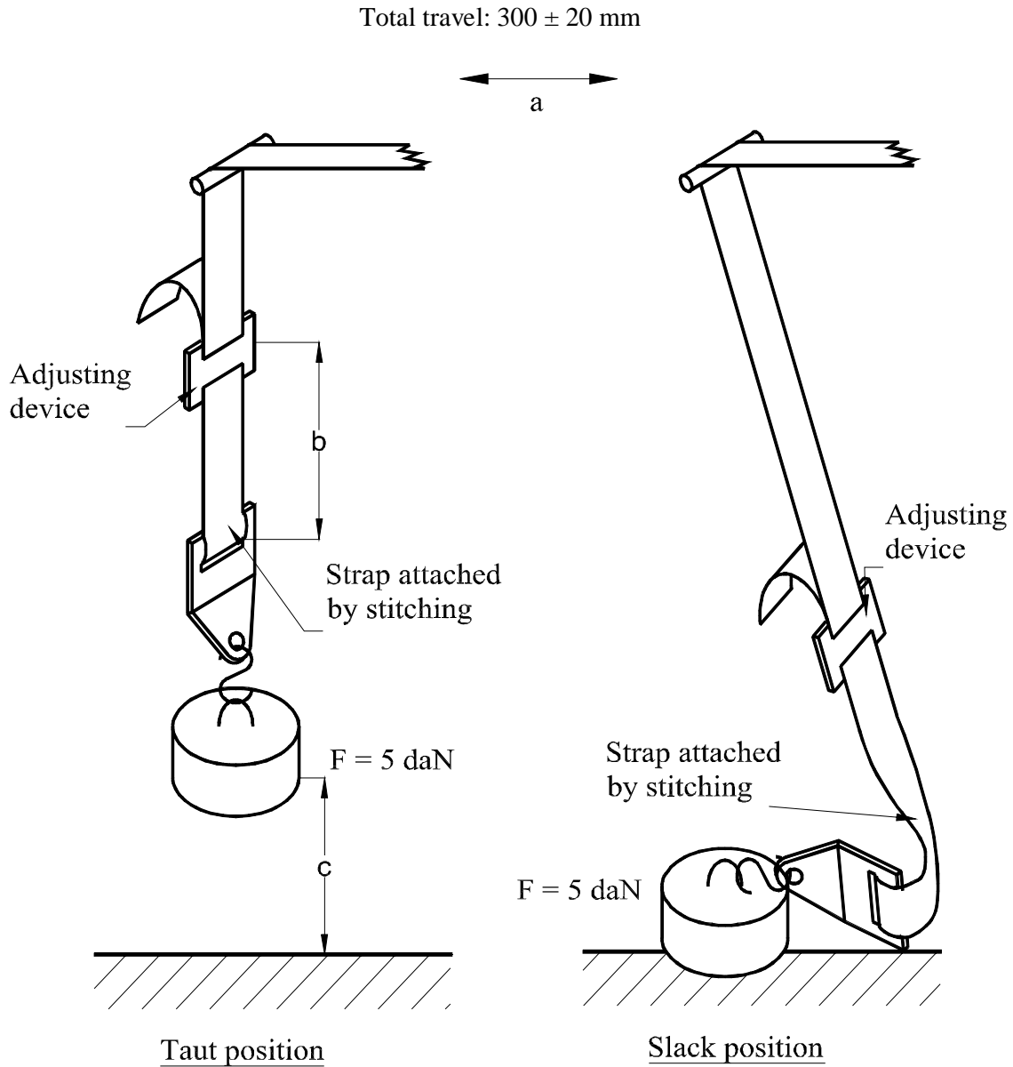
Figure 3: Type 3 procedure and micro-slip test
