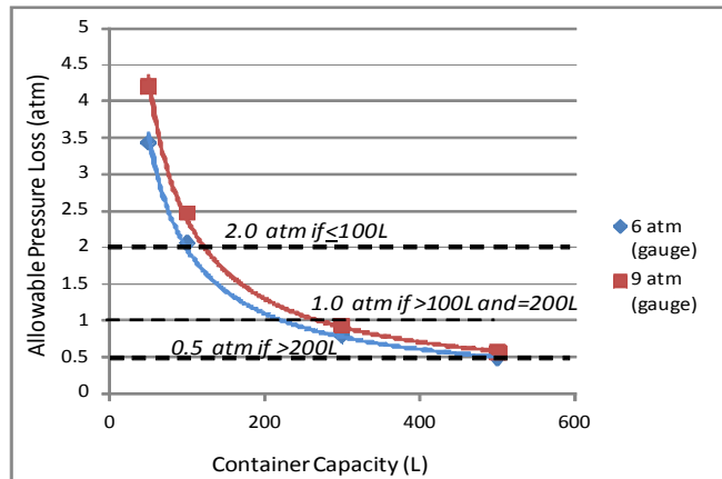
Figure 5. Allowable pressure loss during the LHSS leak test
