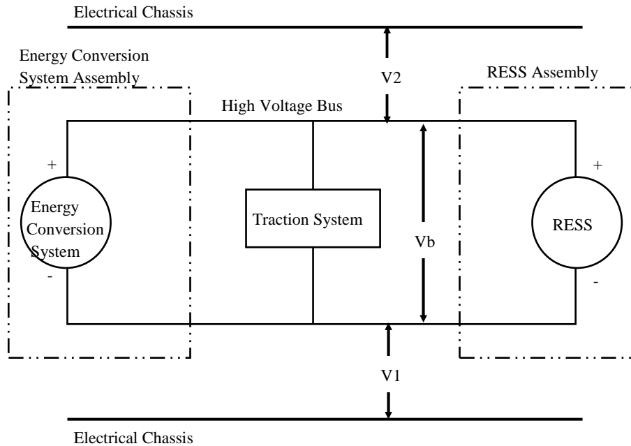
Figure 9 Measurement of V_b , V_1 , V_2
