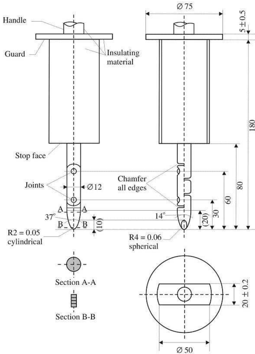
Figure 12 Jointed Test Fingers
