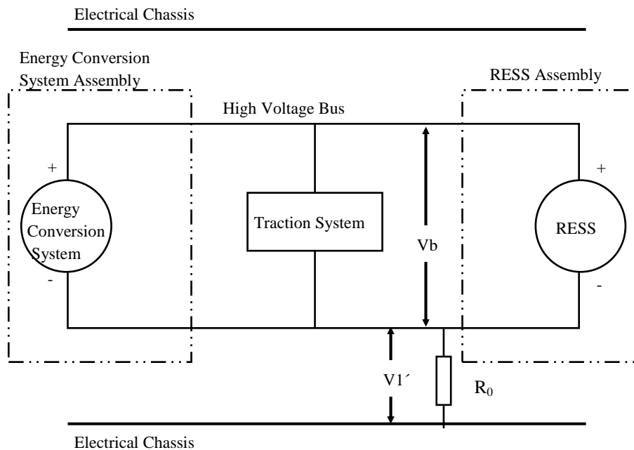
Figure 10 Measurement of V1'
