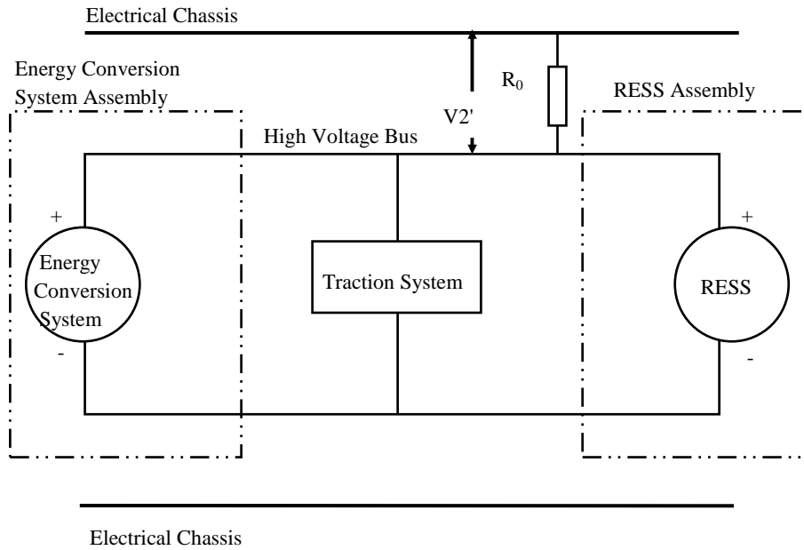
Figure 11 Measurement of V_2
