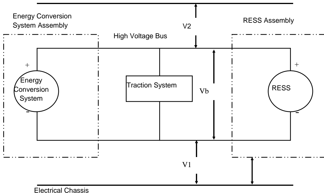
Figure 14 Measurement of V_b , V_1 , V_2
