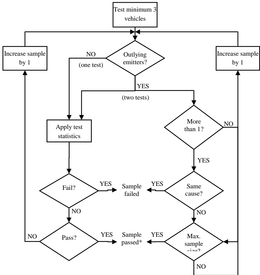
Figure App4/2 In-service conformity testing - selection and test of vehicles
