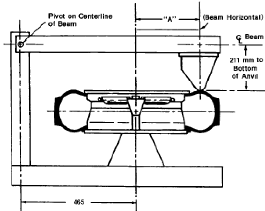
Figure 6 Bead Unseating Fixture (all dimension in mm) and table of "A" dimensions
