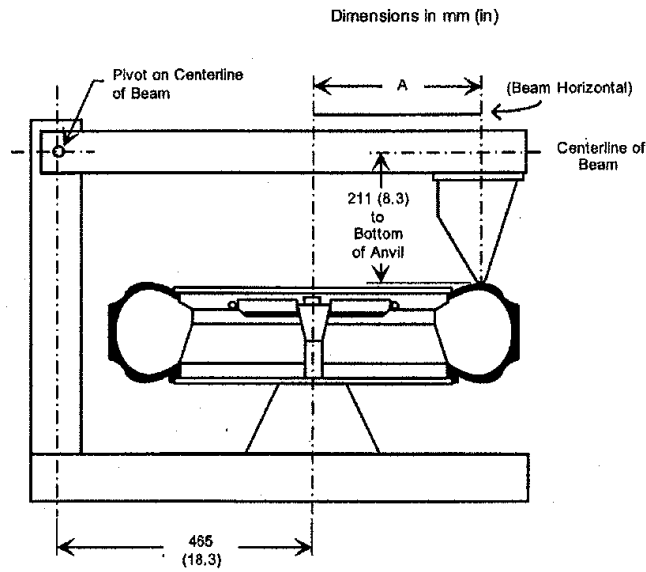
Figure 2 Bead unseating fixture
