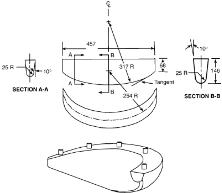
Figure 7 Diagram of bead unseating block (all dimensions in mm)
